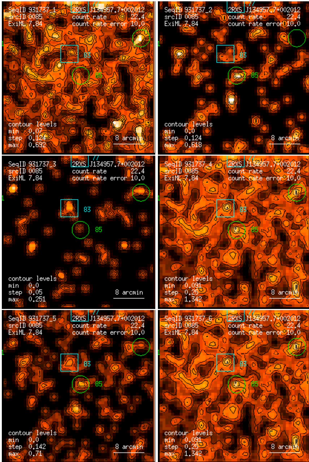
Figure 85: RASS 931737: detection 0085: band rate images, Gaussian filter: (1) PSPC channels 11 – 41, (2) 52 – 90, (3) 91 – 201, (4) 11 – 235, (5) 52 – 201, (6) 11 – 201. Broad band rates in counts/ks. Band rate contour levels in counts/ks/arcmin 2 .
