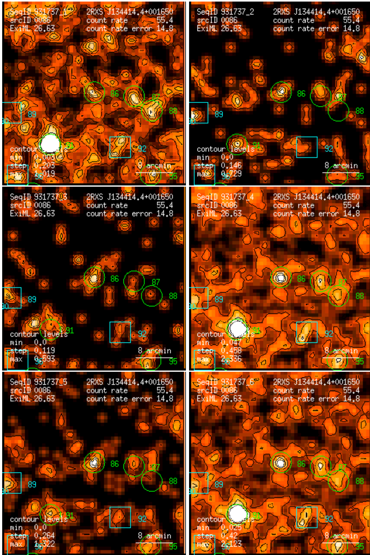
Figure 86: RASS 931737: detection 0086: band rate images, Gaussian filter: (1) PSPC channels 11 – 41, (2) 52 – 90, (3) 91 – 201, (4) 11 – 235, (5) 52 – 201, (6) 11 – 201. Broad band rates in counts/ks. Band rate contour levels in counts/ks/arcmin 2 .
