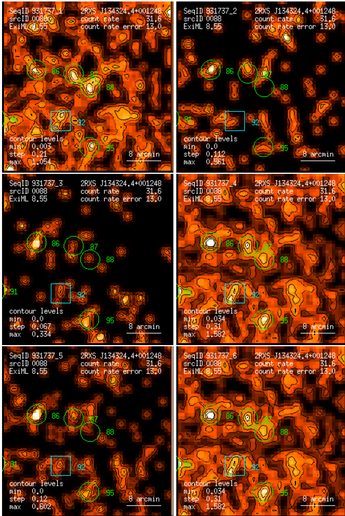
Figure 88: RASS 931737: detection 0088: band rate images, Gaussian filter: (1) PSPC channels 11 – 41, (2) 52 – 90, (3) 91 – 201, (4) 11 – 235, (5) 52 – 201, (6) 11 – 201. Broad band rates in counts/ks. Band rate contour levels in counts/ks/arcmin 2 .
