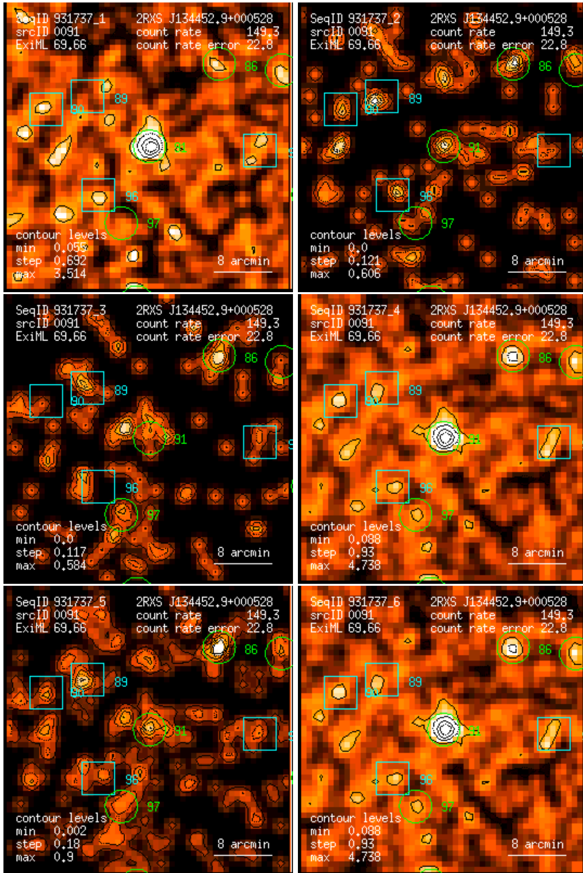
Figure 91: RASS 931737: detection 0091: band rate images, Gaussian filter: (1) PSPC channels 11 – 41, (2) 52 – 90, (3) 91 – 201, (4) 11 – 235, (5) 52 – 201, (6) 11 – 201. Broad band rates in counts/ks. Band rate contour levels in counts/ks/arcmin 2 .
