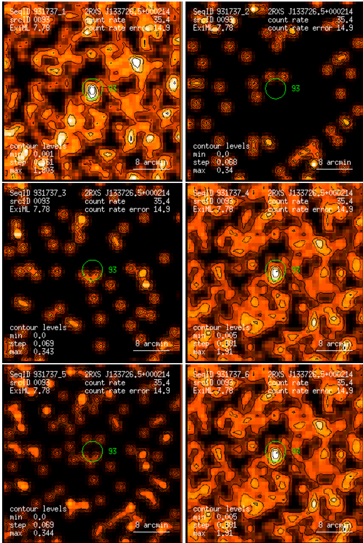
Figure 93: RASS 931737: detection 0093: band rate images, Gaussian filter: (1) PSPC channels 11 – 41, (2) 52 – 90, (3) 91 – 201, (4) 11 – 235, (5) 52 – 201, (6) 11 – 201. Broad band rates in counts/ks. Band rate contour levels in counts/ks/arcmin 2 .
