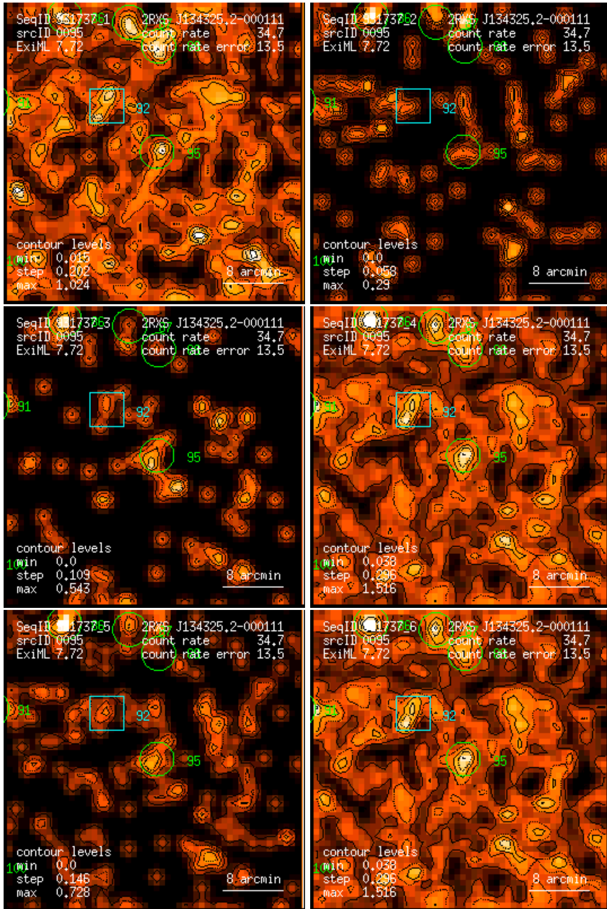
Figure 95: RASS 931737: detection 0095: band rate images, Gaussian filter: (1) PSPC channels 11 – 41, (2) 52 – 90, (3) 91 – 201, (4) 11 – 235, (5) 52 – 201, (6) 11 – 201. Broad band rates in counts/ks. Band rate contour levels in counts/ks/arcmin 2 .
