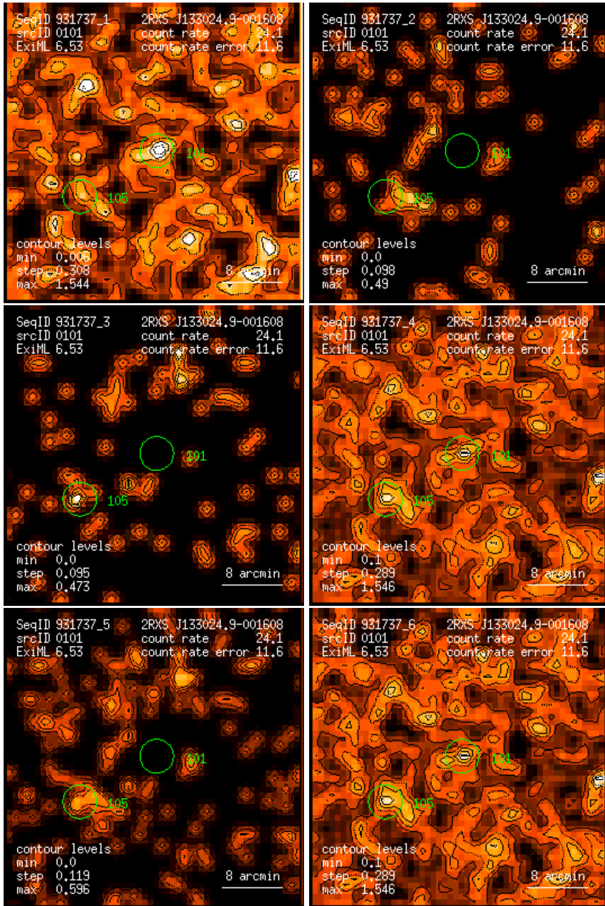
Figure 101: RASS 931737: detection 0101: band rate images, Gaussian filter: (1) PSPC channels 11 – 41, (2) 52 – 90, (3) 91 – 201, (4) 11 – 235, (5) 52 – 201, (6) 11 – 201. Broad band rates in counts/ks. Band rate contour levels in counts/ks/arcmin 2 .
