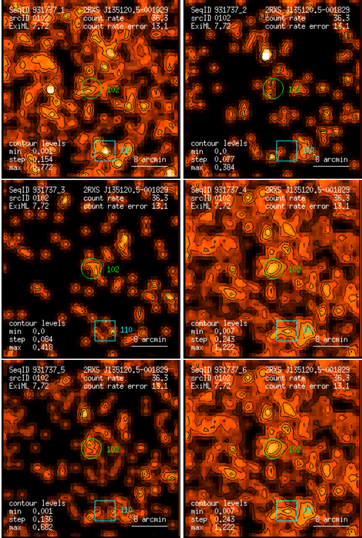
Figure 102: RASS 931737: detection 0102: band rate images, Gaussian filter: (1) PSPC channels 11 – 41, (2) 52 – 90, (3) 91 – 201, (4) 11 – 235, (5) 52 – 201, (6) 11 – 201. Broad band rates in counts/ks. Band rate contour levels in counts/ks/arcmin 2 .
