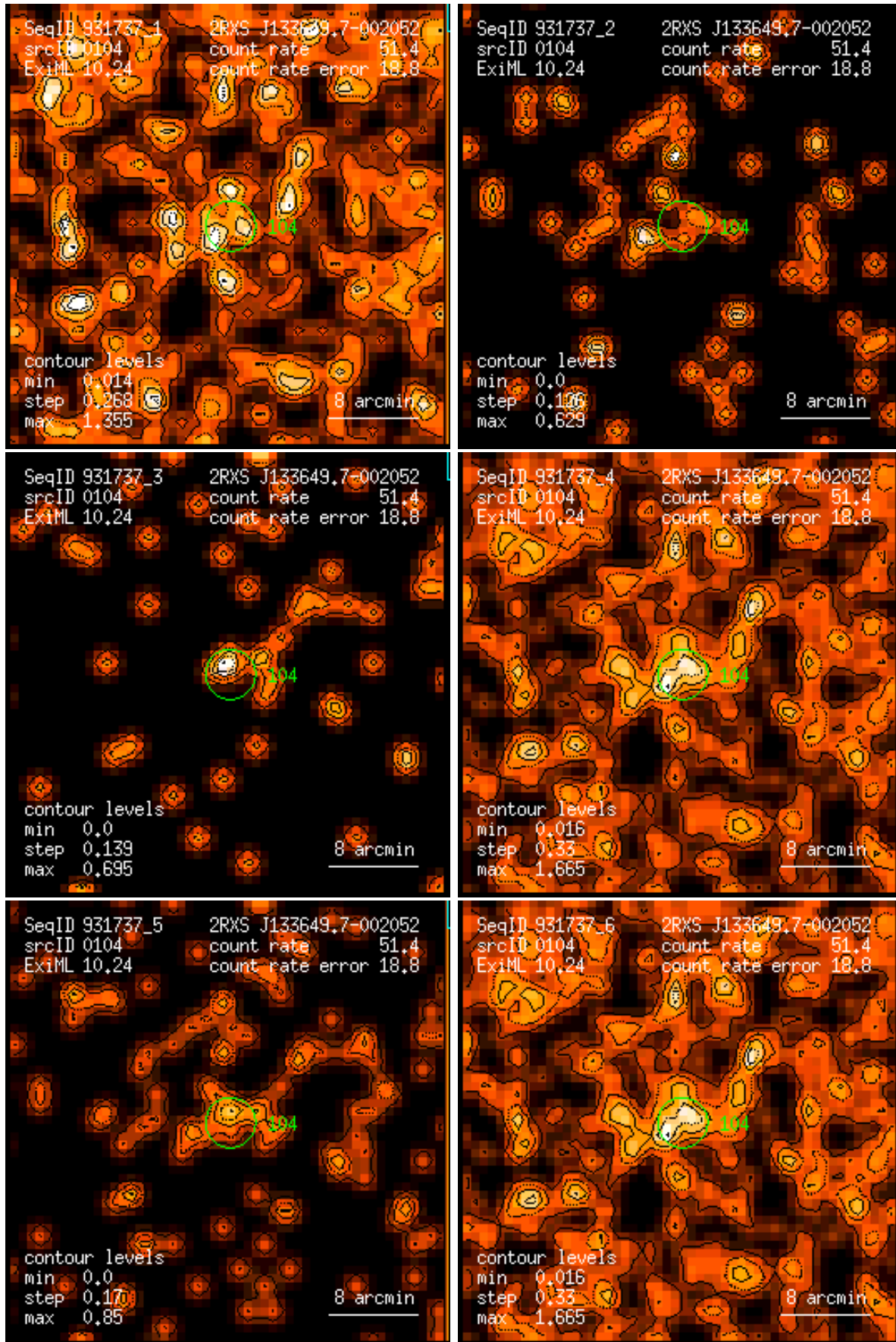
Figure 104: RASS 931737: detection 0104: band rate images, Gaussian filter: (1) PSPC channels 11 – 41, (2) 52 – 90, (3) 91 – 201, (4) 11 – 235, (5) 52 – 201, (6) 11 – 201. Broad band rates in counts/ks. Band rate contour levels in counts/ks/arcmin 2 .
