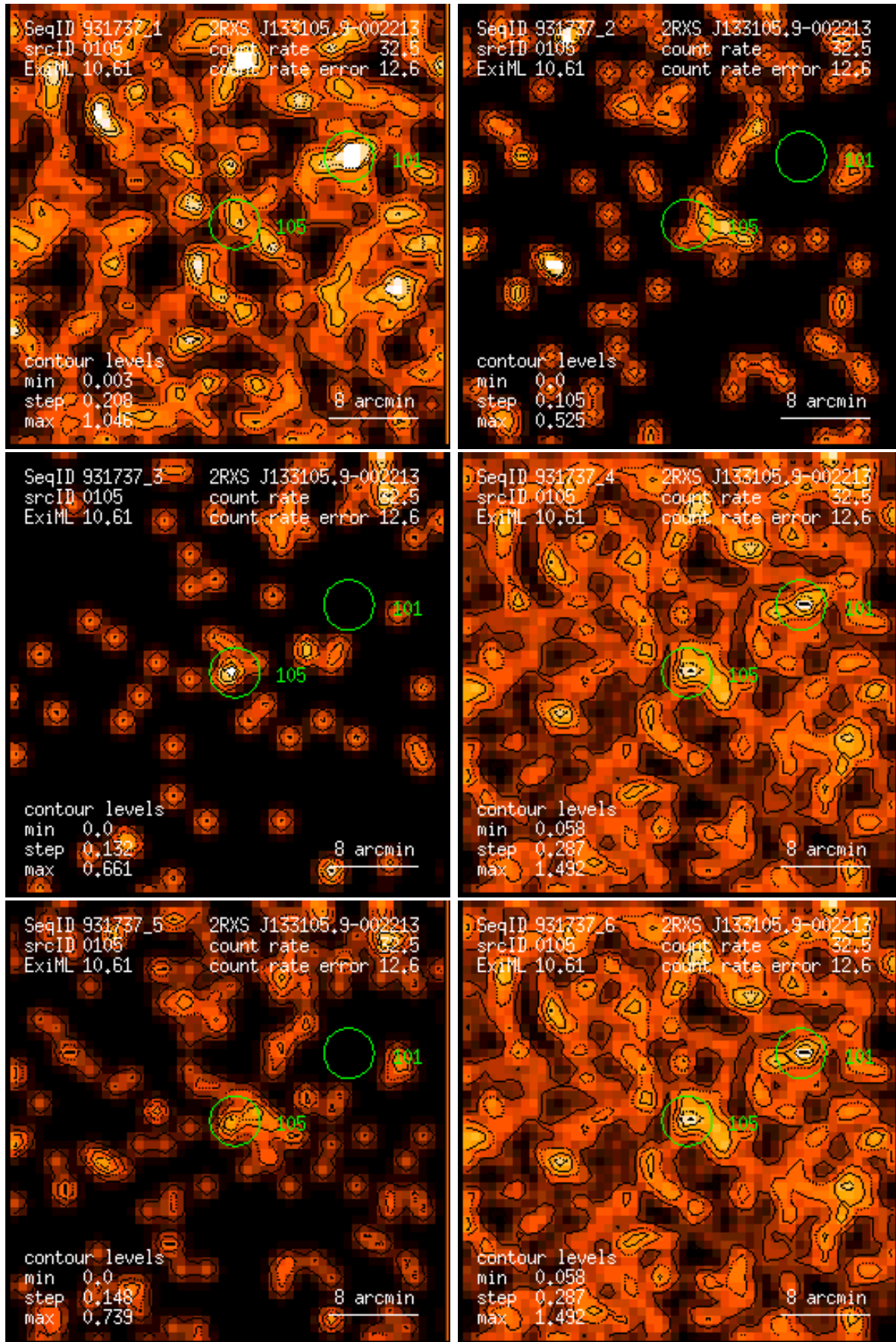
Figure 105: RASS 931737: detection 0105: band rate images, Gaussian filter: (1) PSPC channels 11 – 41, (2) 52 – 90, (3) 91 – 201, (4) 11 – 235, (5) 52 – 201, (6) 11 – 201. Broad band rates in counts/ks. Band rate contour levels in counts/ks/arcmin 2 .
