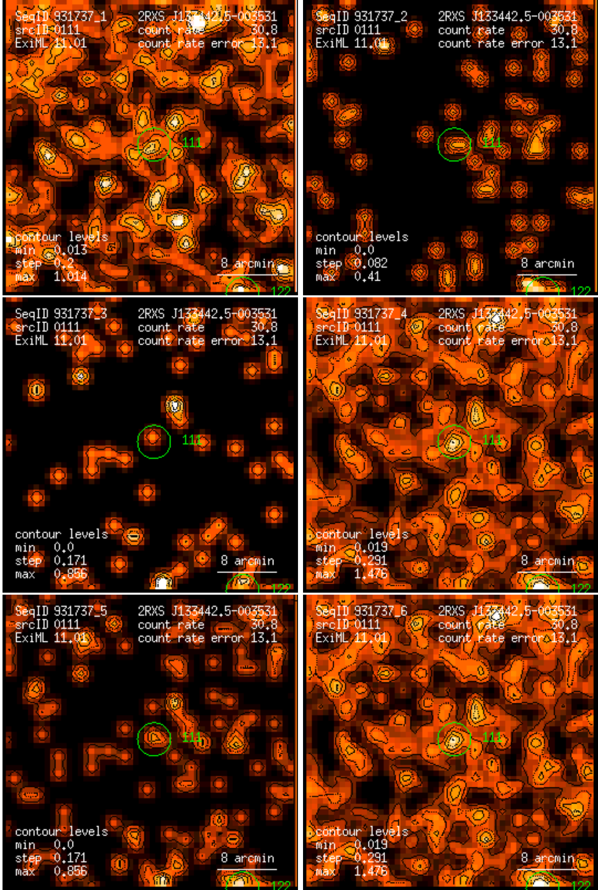
Figure 111: RASS 931737: detection 0111: band rate images, Gaussian filter: (1) PSPC channels 11 – 41, (2) 52 – 90, (3) 91 – 201, (4) 11 – 235, (5) 52 – 201, (6) 11 – 201. Broad band rates in counts/ks. Band rate contour levels in counts/ks/arcmin 2 .
