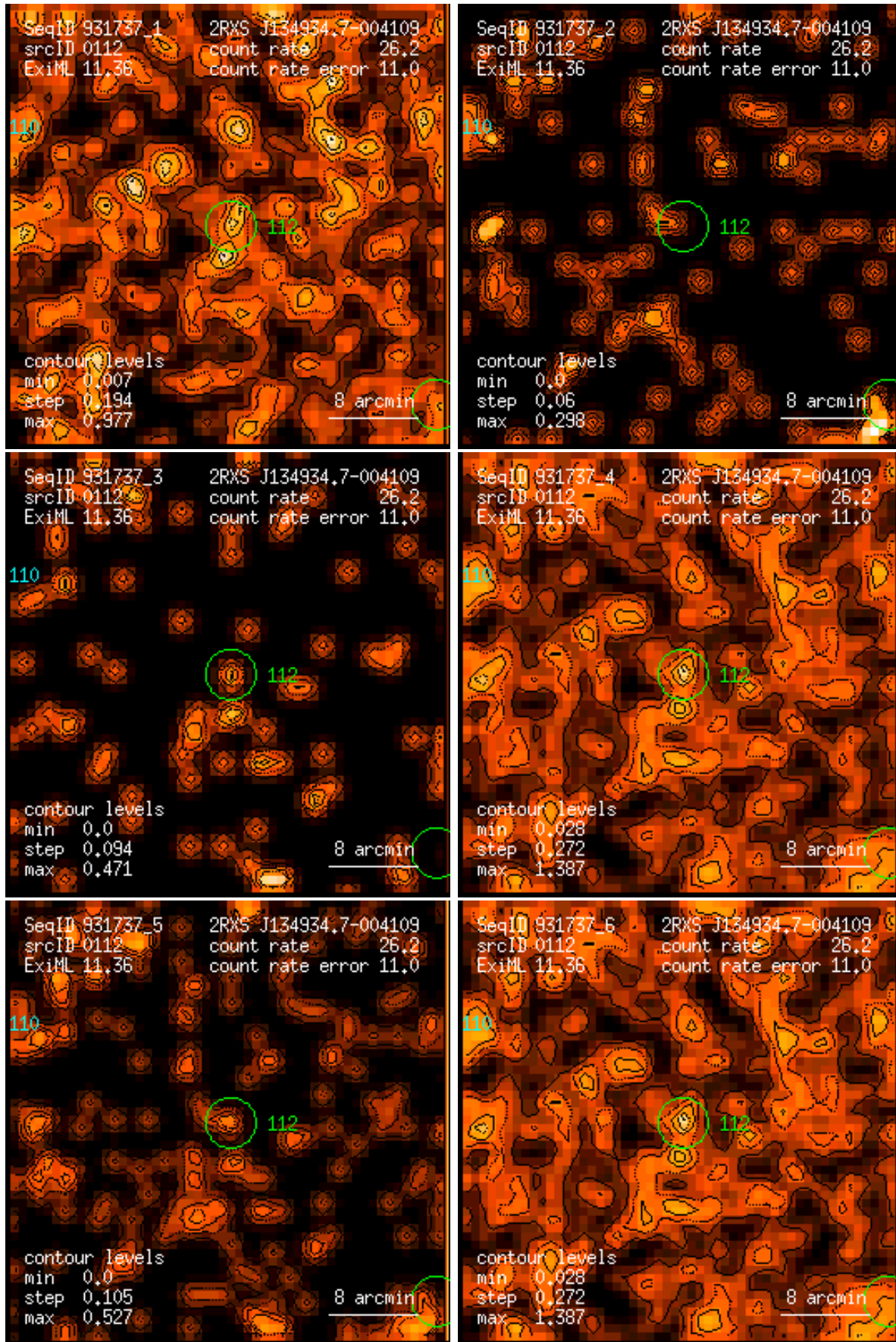
Figure 112: RASS 931737: detection 0112: band rate images, Gaussian filter: (1) PSPC channels 11 – 41, (2) 52 – 90, (3) 91 – 201, (4) 11 – 235, (5) 52 – 201, (6) 11 – 201. Broad band rates in counts/ks. Band rate contour levels in counts/ks/arcmin 2 .
