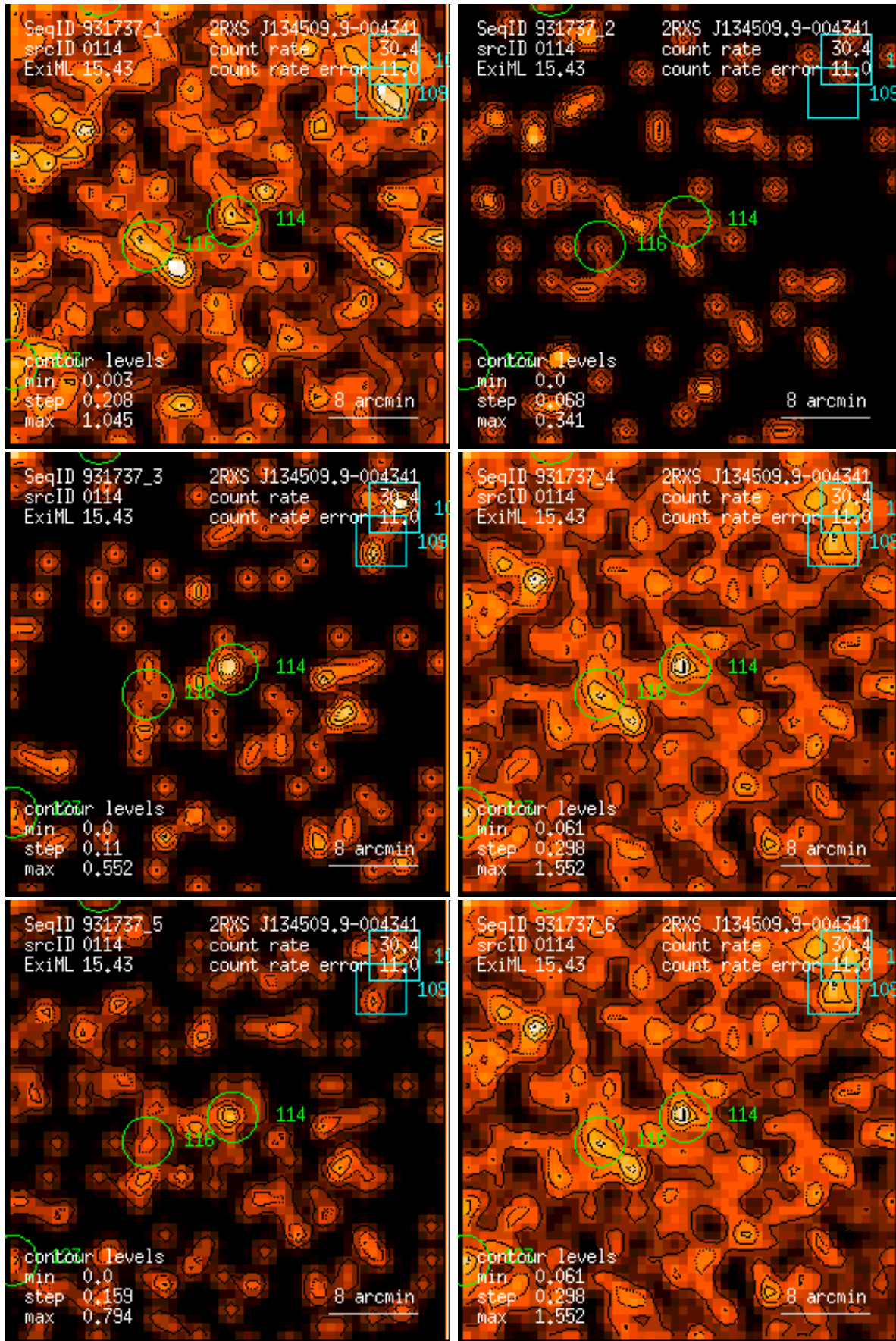
Figure 114: RASS 931737: detection 0114: band rate images, Gaussian filter: (1) PSPC channels 11 – 41, (2) 52 – 90, (3) 91 – 201, (4) 11 – 235, (5) 52 – 201, (6) 11 – 201. Broad band rates in counts/ks. Band rate contour levels in counts/ks/arcmin 2 .
