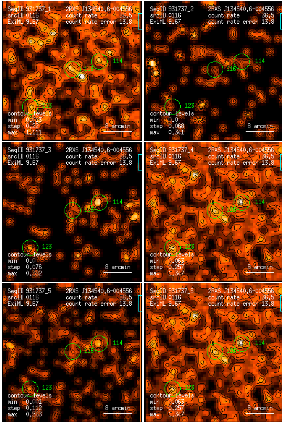
Figure 116: RASS 931737: detection 0116: band rate images, Gaussian filter: (1) PSPC channels 11 – 41, (2) 52 – 90, (3) 91 – 201, (4) 11 – 235, (5) 52 – 201, (6) 11 – 201. Broad band rates in counts/ks. Band rate contour levels in counts/ks/arcmin 2 .
