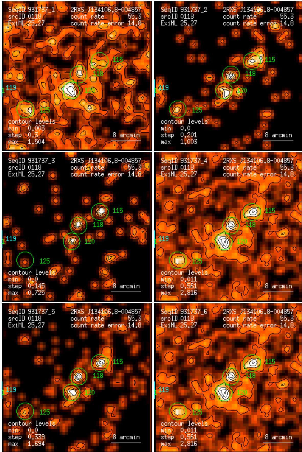
Figure 118: RASS 931737: detection 0118: band rate images, Gaussian filter: (1) PSPC channels 11 – 41, (2) 52 – 90, (3) 91 – 201, (4) 11 – 235, (5) 52 – 201, (6) 11 – 201. Broad band rates in counts/ks. Band rate contour levels in counts/ks/arcmin 2 .
