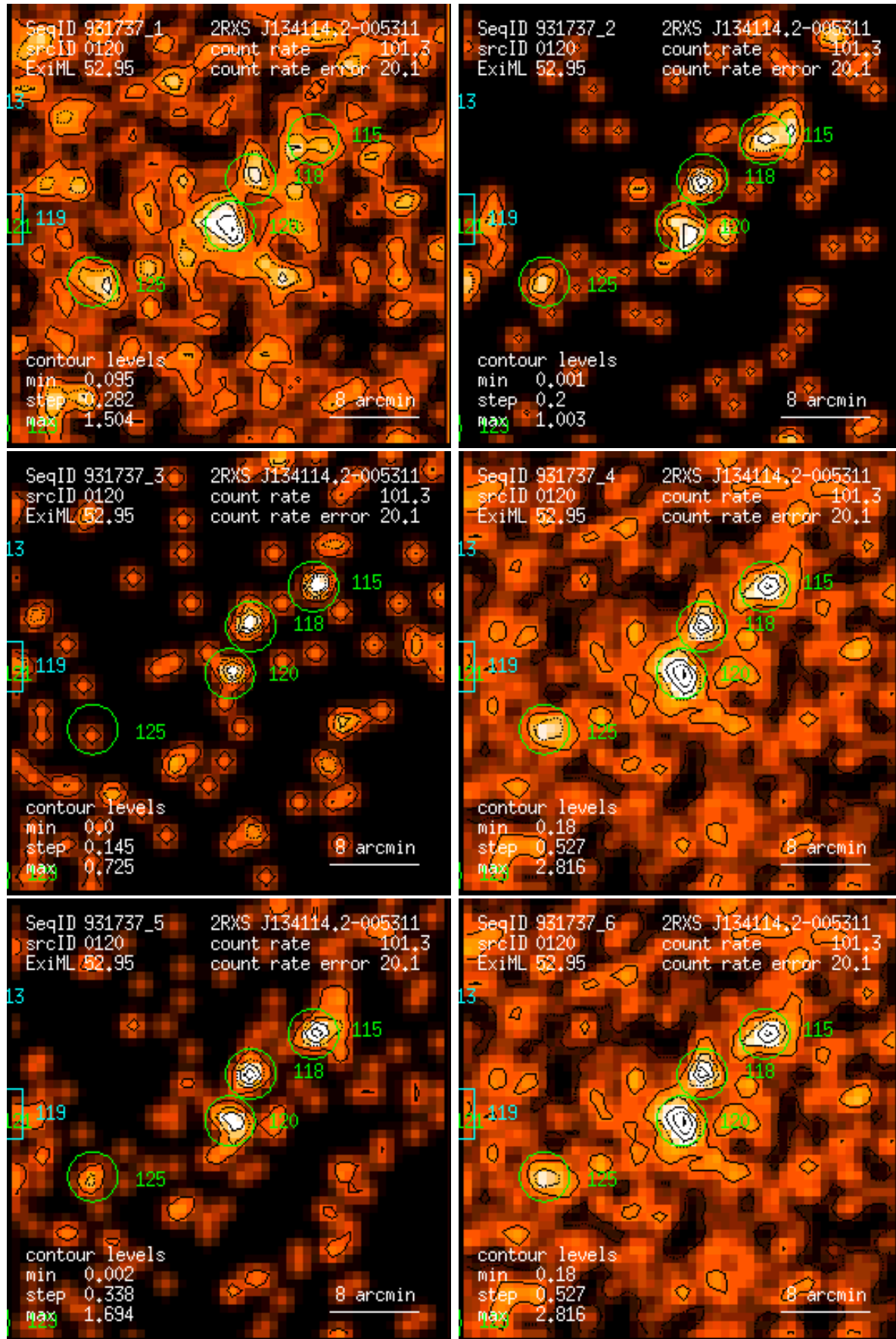
Figure 120: RASS 931737: detection 0120: band rate images, Gaussian filter: (1) PSPC channels 11 – 41, (2) 52 – 90, (3) 91 – 201, (4) 11 – 235, (5) 52 – 201, (6) 11 – 201. Broad band rates in counts/ks. Band rate contour levels in counts/ks/arcmin 2 .
