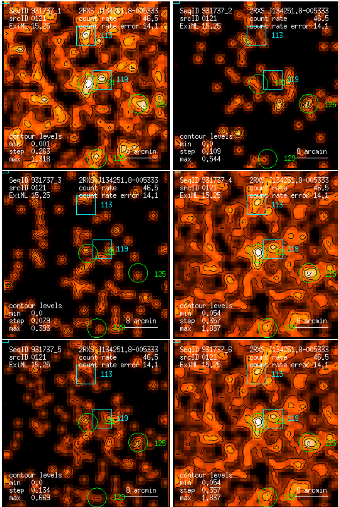
Figure 121: RASS 931737: detection 0121: band rate images, Gaussian filter: (1) PSPC channels 11 – 41, (2) 52 – 90, (3) 91 – 201, (4) 11 – 235, (5) 52 – 201, (6) 11 – 201. Broad band rates in counts/ks. Band rate contour levels in counts/ks/arcmin 2 .
