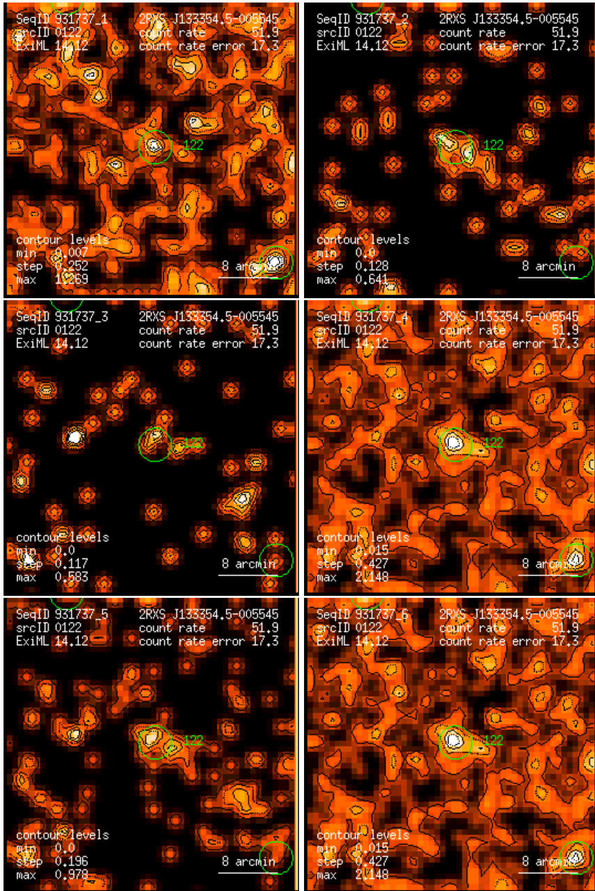
Figure 122: RASS 931737: detection 0122: band rate images, Gaussian filter: (1) PSPC channels 11 – 41, (2) 52 – 90, (3) 91 – 201, (4) 11 – 235, (5) 52 – 201, (6) 11 – 201. Broad band rates in counts/ks. Band rate contour levels in counts/ks/arcmin 2 .
