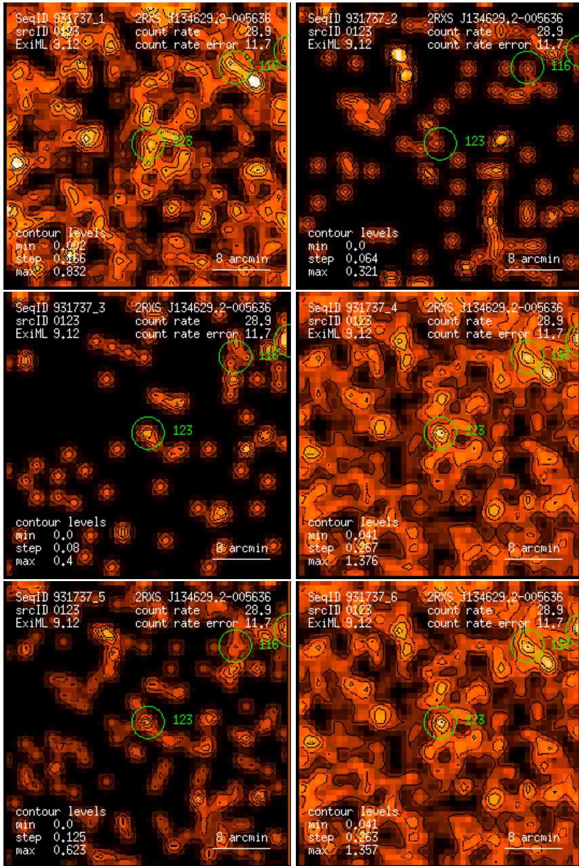
Figure 123: RASS 931737: detection 0123: band rate images, Gaussian filter: (1) PSPC channels 11 – 41, (2) 52 – 90, (3) 91 – 201, (4) 11 – 235, (5) 52 – 201, (6) 11 – 201. Broad band rates in counts/ks. Band rate contour levels in counts/ks/arcmin 2 .
