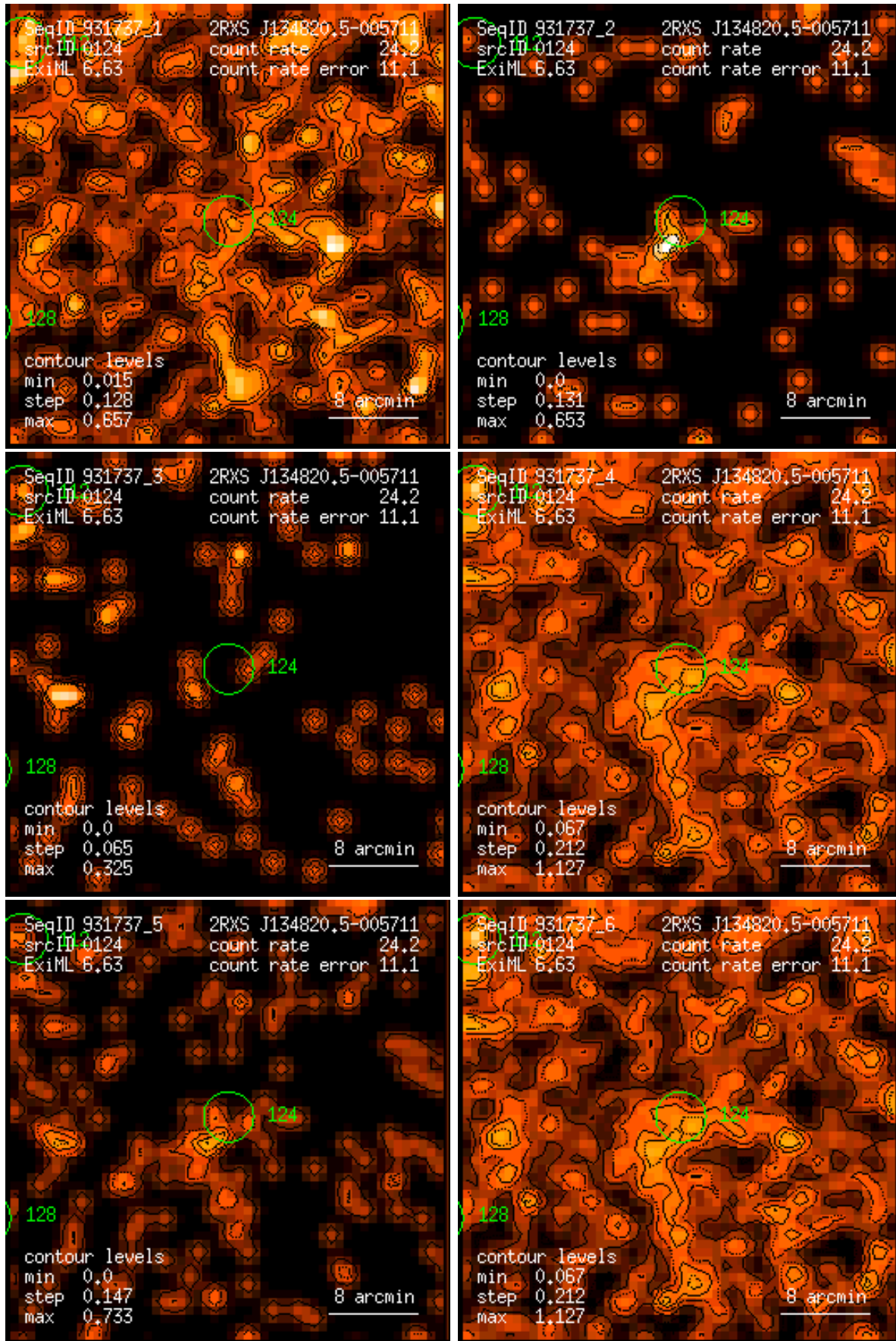
Figure 124: RASS 931737: detection 0124: band rate images, Gaussian filter: (1) PSPC channels 11 – 41, (2) 52 – 90, (3) 91 – 201, (4) 11 – 235, (5) 52 – 201, (6) 11 – 201. Broad band rates in counts/ks. Band rate contour levels in counts/ks/arcmin 2 .
