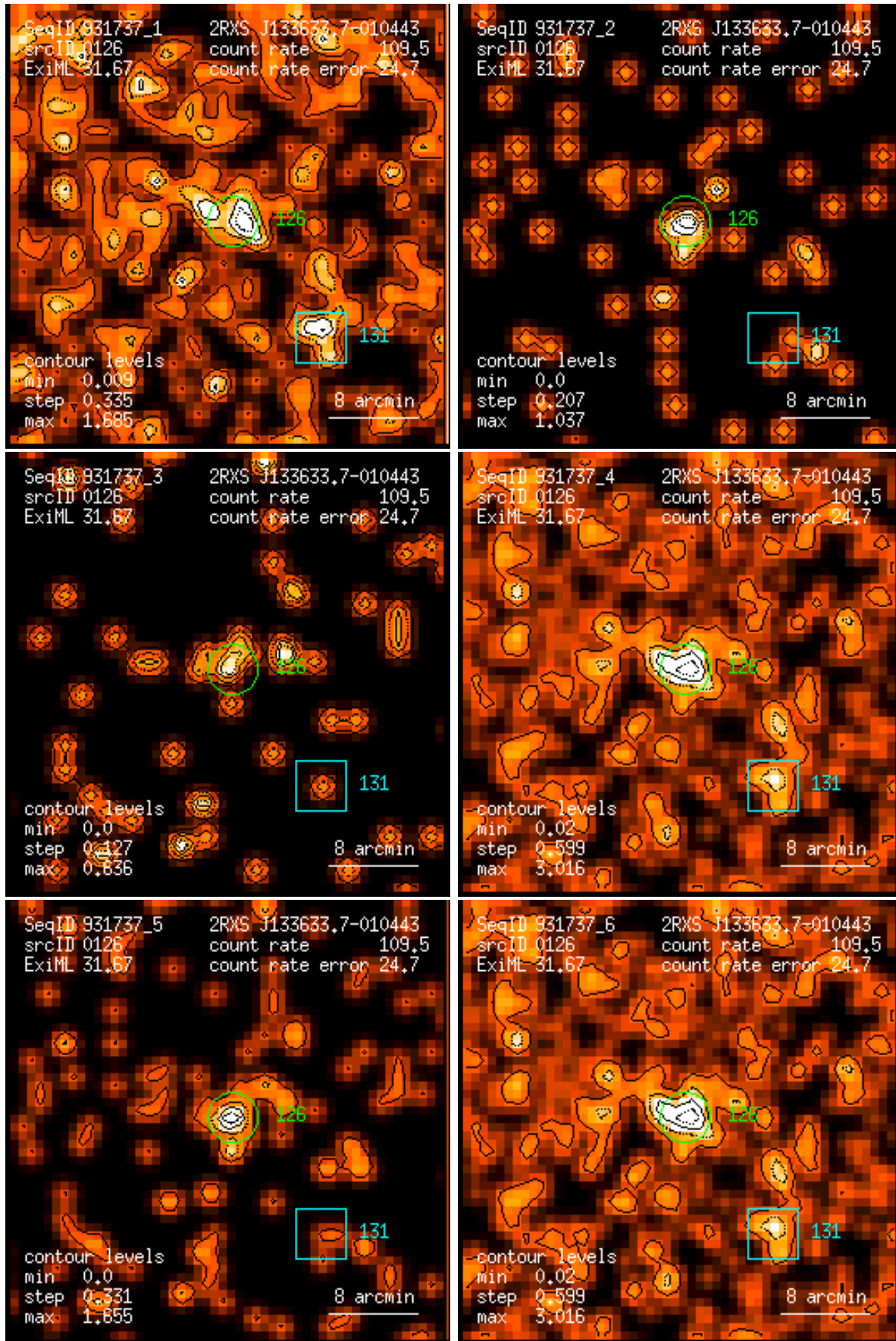
Figure 126: RASS 931737: detection 0126: band rate images, Gaussian filter: (1) PSPC channels 11 – 41, (2) 52 – 90, (3) 91 – 201, (4) 11 – 235, (5) 52 – 201, (6) 11 – 201. Broad band rates in counts/ks. Band rate contour levels in counts/ks/arcmin 2 .
