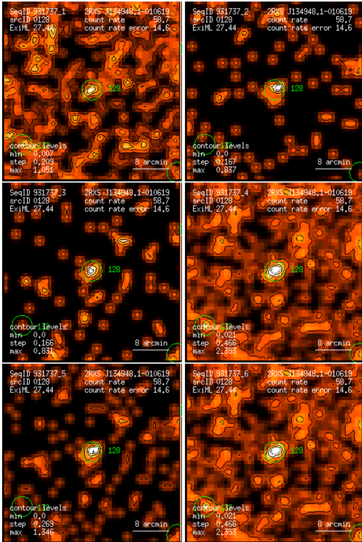
Figure 128: RASS 931737: detection 0128: band rate images, Gaussian filter: (1) PSPC channels 11 – 41, (2) 52 – 90, (3) 91 – 201, (4) 11 – 235, (5) 52 – 201, (6) 11 – 201. Broad band rates in counts/ks. Band rate contour levels in counts/ks/arcmin 2 .
