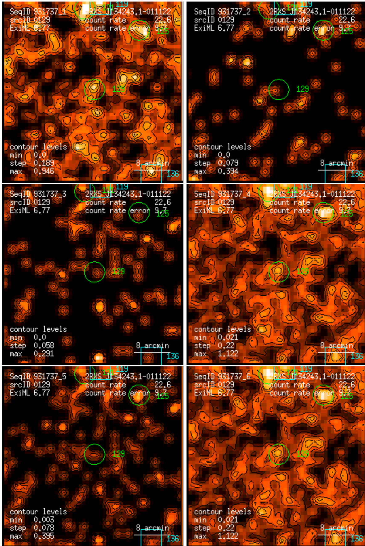
Figure 129: RASS 931737: detection 0129: band rate images, Gaussian filter: (1) PSPC channels 11 – 41, (2) 52 – 90, (3) 91 – 201, (4) 11 – 235, (5) 52 – 201, (6) 11 – 201. Broad band rates in counts/ks. Band rate contour levels in counts/ks/arcmin 2 .
