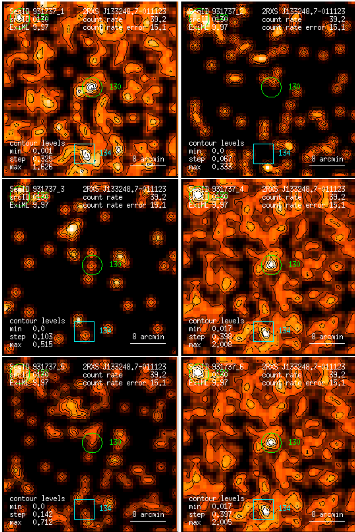
Figure 130: RASS 931737: detection 0130: band rate images, Gaussian filter: (1) PSPC channels 11 – 41, (2) 52 – 90, (3) 91 – 201, (4) 11 – 235, (5) 52 – 201, (6) 11 – 201. Broad band rates in counts/ks. Band rate contour levels in counts/ks/arcmin 2 .
