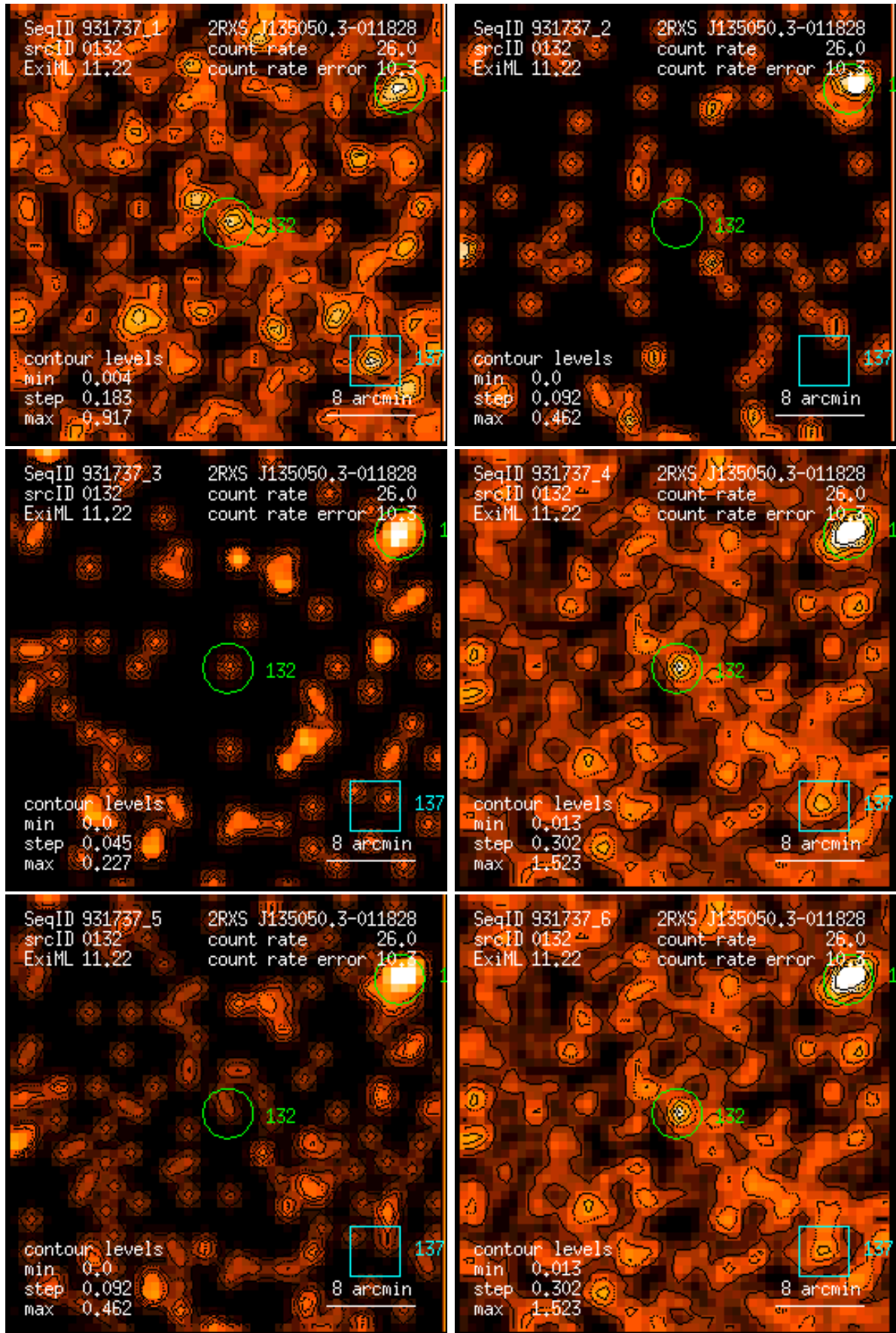
Figure 132: RASS 931737: detection 0132: band rate images, Gaussian filter: (1) PSPC channels 11 – 41, (2) 52 – 90, (3) 91 – 201, (4) 11 – 235, (5) 52 – 201, (6) 11 – 201. Broad band rates in counts/ks. Band rate contour levels in counts/ks/arcmin 2 .
