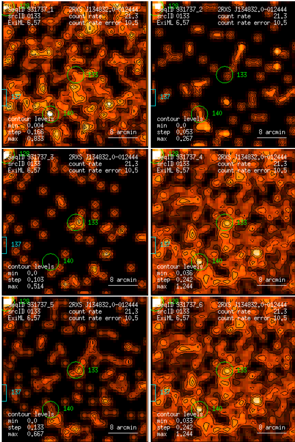
Figure 133: RASS 931737: detection 0133: band rate images, Gaussian filter: (1) PSPC channels 11 – 41, (2) 52 – 90, (3) 91 – 201, (4) 11 – 235, (5) 52 – 201, (6) 11 – 201. Broad band rates in counts/ks. Band rate contour levels in counts/ks/arcmin 2 .
