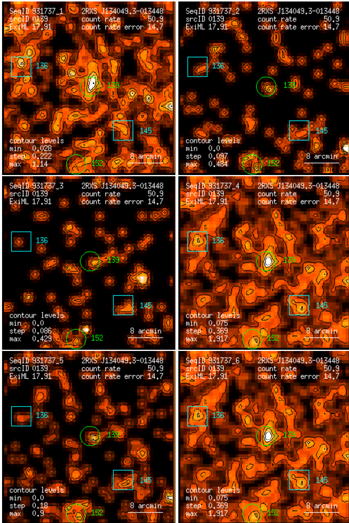
Figure 139: RASS 931737: detection 0139: band rate images, Gaussian filter: (1) PSPC channels 11 – 41, (2) 52 – 90, (3) 91 – 201, (4) 11 – 235, (5) 52 – 201, (6) 11 – 201. Broad band rates in counts/ks. Band rate contour levels in counts/ks/arcmin 2 .
