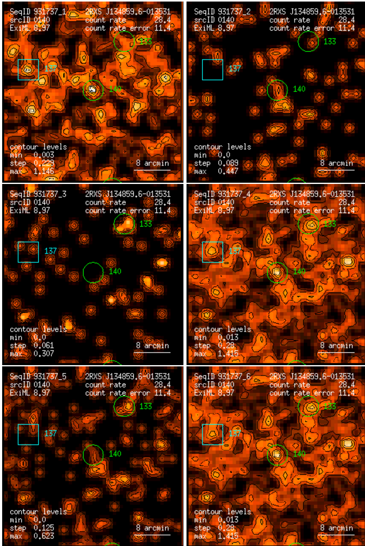
Figure 140: RASS 931737: detection 0140: band rate images, Gaussian filter: (1) PSPC channels 11 – 41, (2) 52 – 90, (3) 91 – 201, (4) 11 – 235, (5) 52 – 201, (6) 11 – 201. Broad band rates in counts/ks. Band rate contour levels in counts/ks/arcmin 2 .
