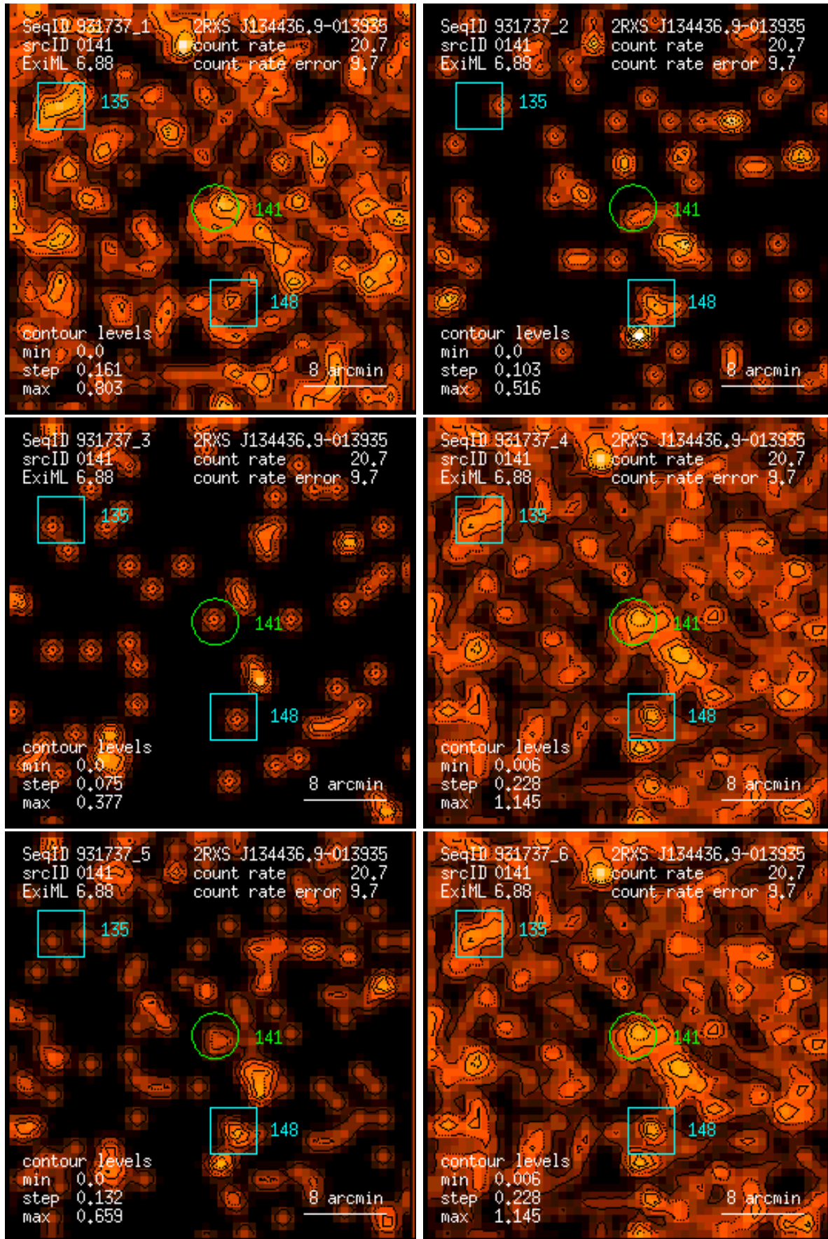
Figure 141: RASS 931737: detection 0141: band rate images, Gaussian filter: (1) PSPC channels 11 – 41, (2) 52 – 90, (3) 91 – 201, (4) 11 – 235, (5) 52 – 201, (6) 11 – 201. Broad band rates in counts/ks. Band rate contour levels in counts/ks/arcmin 2 .
