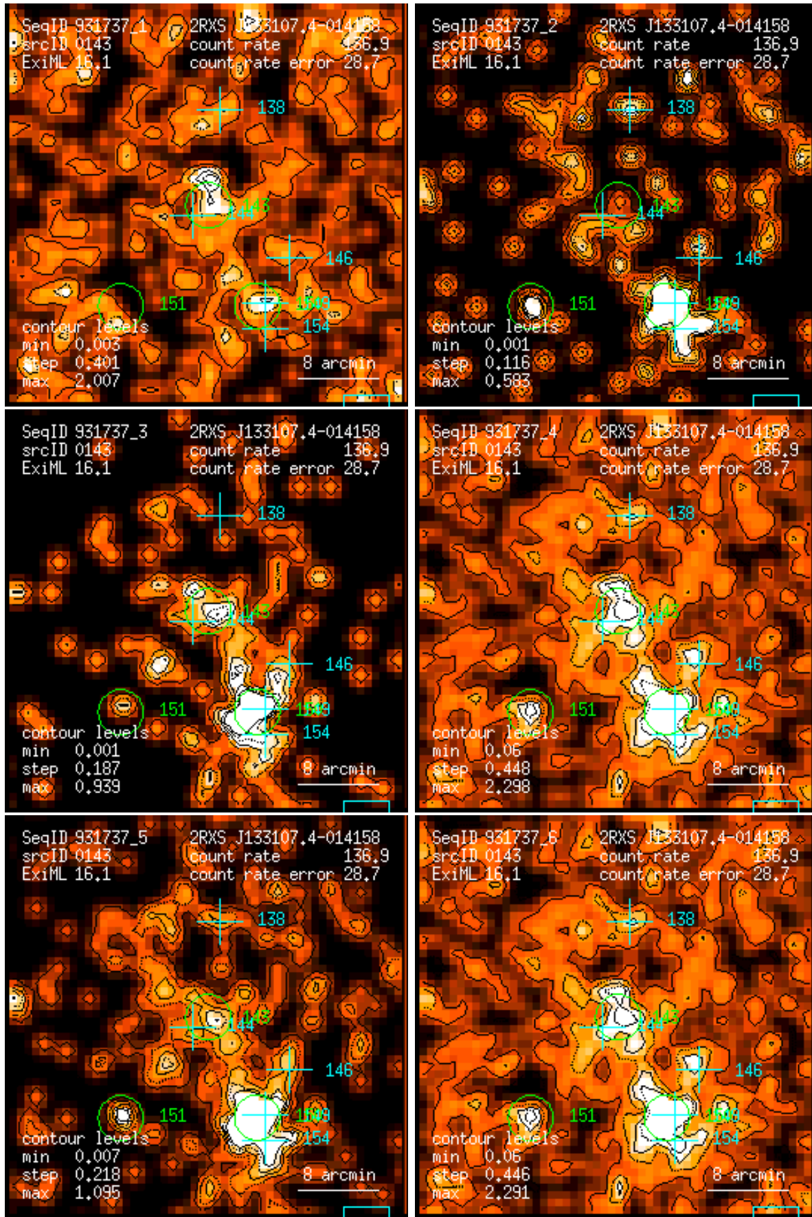
Figure 143: RASS 931737: detection 0143: band rate images, Gaussian filter: (1) PSPC channels 11 – 41, (2) 52 – 90, (3) 91 – 201, (4) 11 – 235, (5) 52 – 201, (6) 11 – 201. Broad band rates in counts/ks. Band rate contour levels in counts/ks/arcmin 2 .
