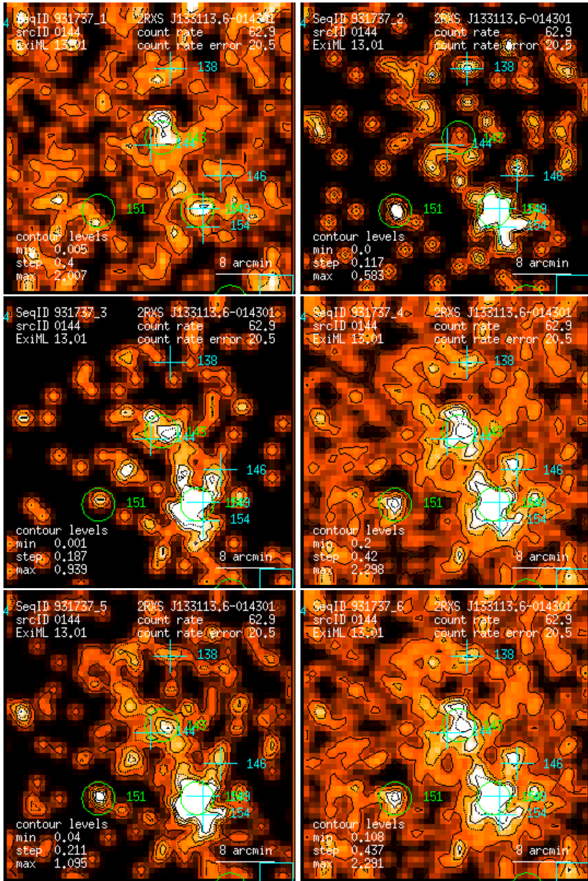
Figure 144: RASS 931737: detection 0144: band rate images, Gaussian filter: (1) PSPC channels 11 – 41, (2) 52 – 90, (3) 91 – 201, (4) 11 – 235, (5) 52 – 201, (6) 11 – 201. Broad band rates in counts/ks. Band rate contour levels in counts/ks/arcmin 2 .
