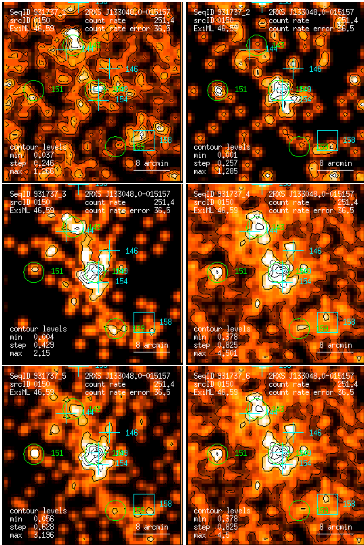
Figure 150: RASS 931737: detection 0150: band rate images, Gaussian filter: (1) PSPC channels 11 – 41, (2) 52 – 90, (3) 91 – 201, (4) 11 – 235, (5) 52 – 201, (6) 11 – 201. Broad band rates in counts/ks. Band rate contour levels in counts/ks/arcmin 2 .
