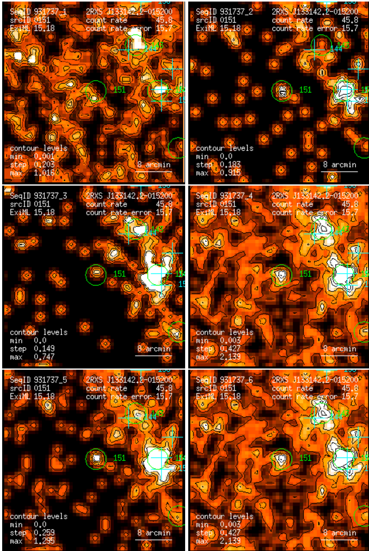
Figure 151: RASS 931737: detection 0151: band rate images, Gaussian filter: (1) PSPC channels 11 – 41, (2) 52 – 90, (3) 91 – 201, (4) 11 – 235, (5) 52 – 201, (6) 11 – 201. Broad band rates in counts/ks. Band rate contour levels in counts/ks/arcmin 2 .
