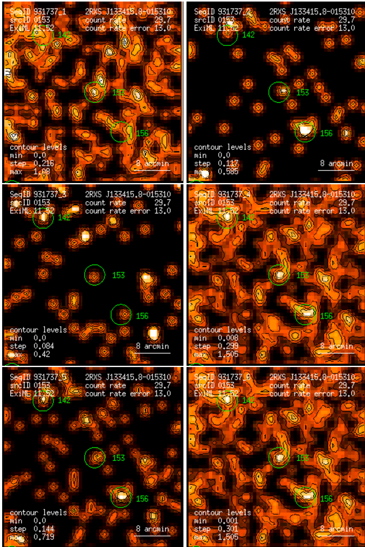
Figure 153: RASS 931737: detection 0153: band rate images, Gaussian filter: (1) PSPC channels 11 – 41, (2) 52 – 90, (3) 91 – 201, (4) 11 – 235, (5) 52 – 201, (6) 11 – 201. Broad band rates in counts/ks. Band rate contour levels in counts/ks/arcmin 2 .
