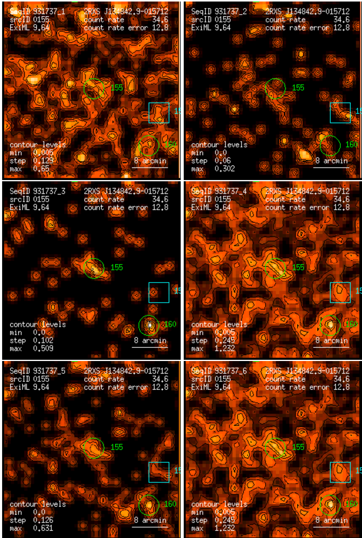
Figure 155: RASS 931737: detection 0155: band rate images, Gaussian filter: (1) PSPC channels 11 – 41, (2) 52 – 90, (3) 91 – 201, (4) 11 – 235, (5) 52 – 201, (6) 11 – 201. Broad band rates in counts/ks. Band rate contour levels in counts/ks/arcmin 2 .
