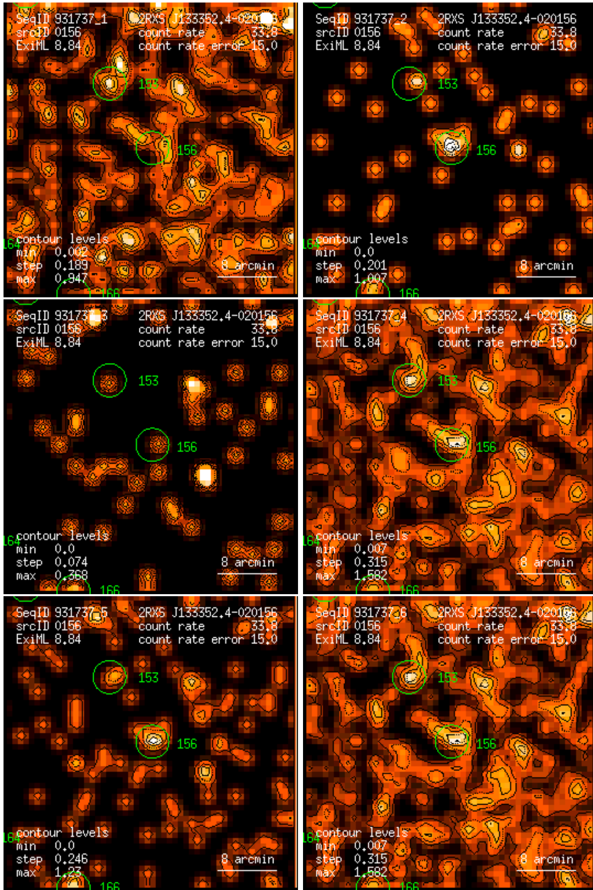
Figure 156: RASS 931737: detection 0156: band rate images, Gaussian filter: (1) PSPC channels 11 – 41, (2) 52 – 90, (3) 91 – 201, (4) 11 – 235, (5) 52 – 201, (6) 11 – 201. Broad band rates in counts/ks. Band rate contour levels in counts/ks/arcmin 2 .
