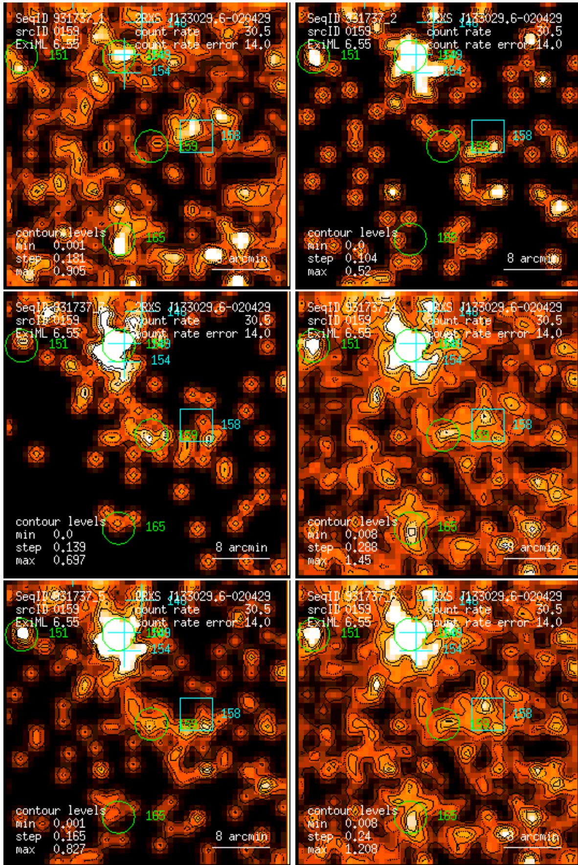
Figure 159: RASS 931737: detection 0159: band rate images, Gaussian filter: (1) PSPC channels 11 – 41, (2) 52 – 90, (3) 91 – 201, (4) 11 – 235, (5) 52 – 201, (6) 11 – 201. Broad band rates in counts/ks. Band rate contour levels in counts/ks/arcmin 2 .
