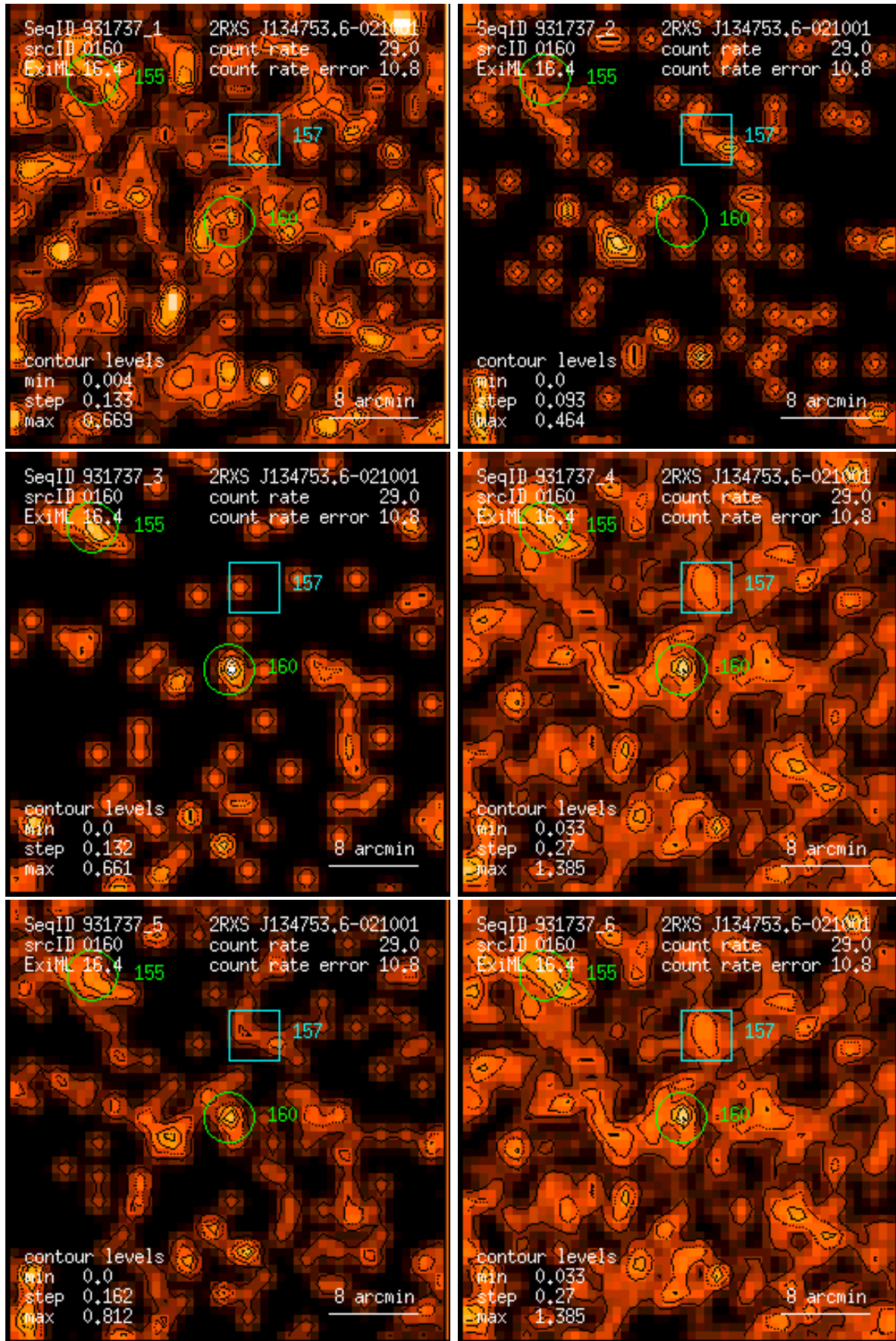
Figure 160: RASS 931737: detection 0160: band rate images, Gaussian filter: (1) PSPC channels 11 – 41, (2) 52 – 90, (3) 91 – 201, (4) 11 – 235, (5) 52 – 201, (6) 11 – 201. Broad band rates in counts/ks. Band rate contour levels in counts/ks/arcmin 2 .
