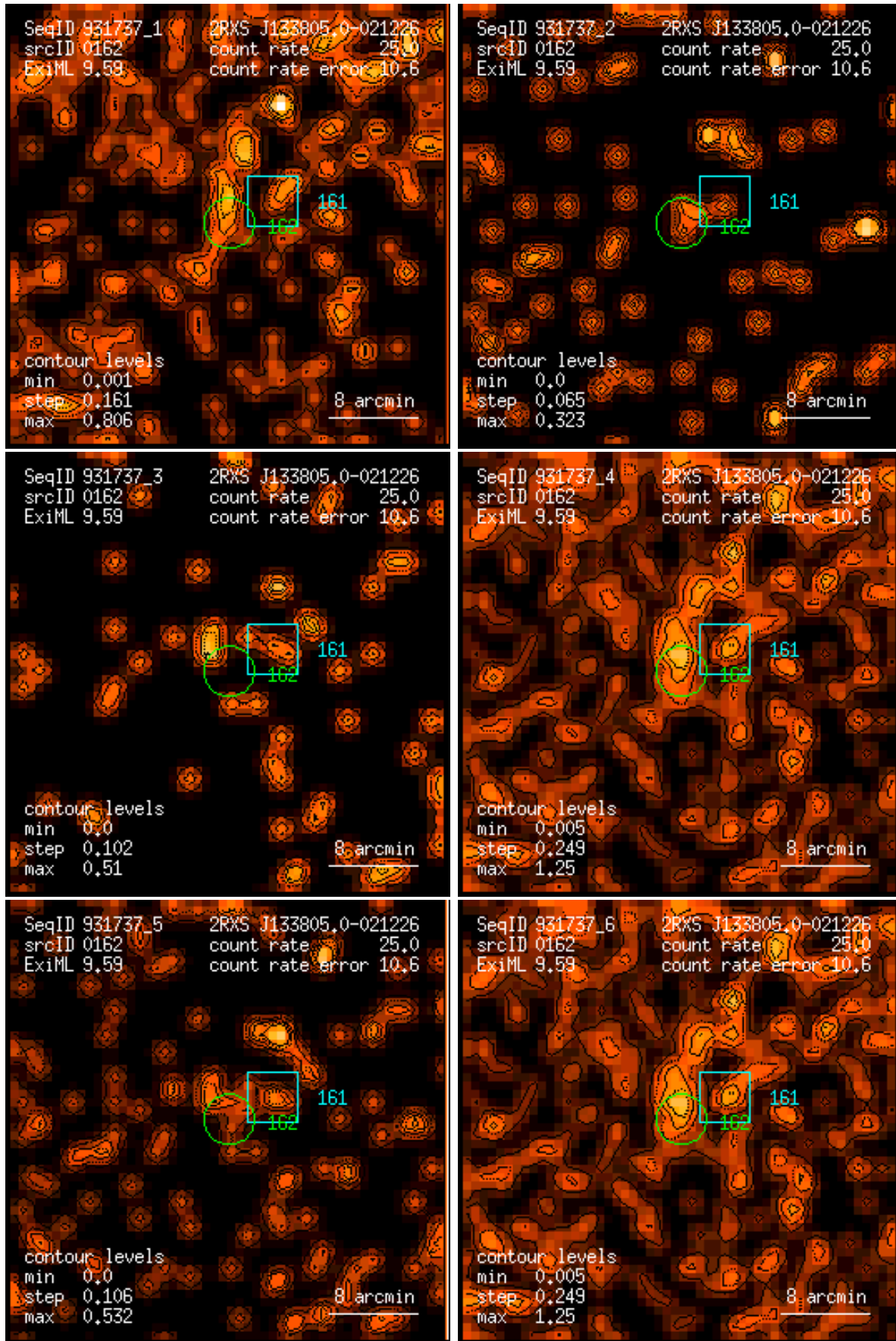
Figure 162: RASS 931737: detection 0162: band rate images, Gaussian filter: (1) PSPC channels 11 – 41, (2) 52 – 90, (3) 91 – 201, (4) 11 – 235, (5) 52 – 201, (6) 11 – 201. Broad band rates in counts/ks. Band rate contour levels in counts/ks/arcmin 2 .
