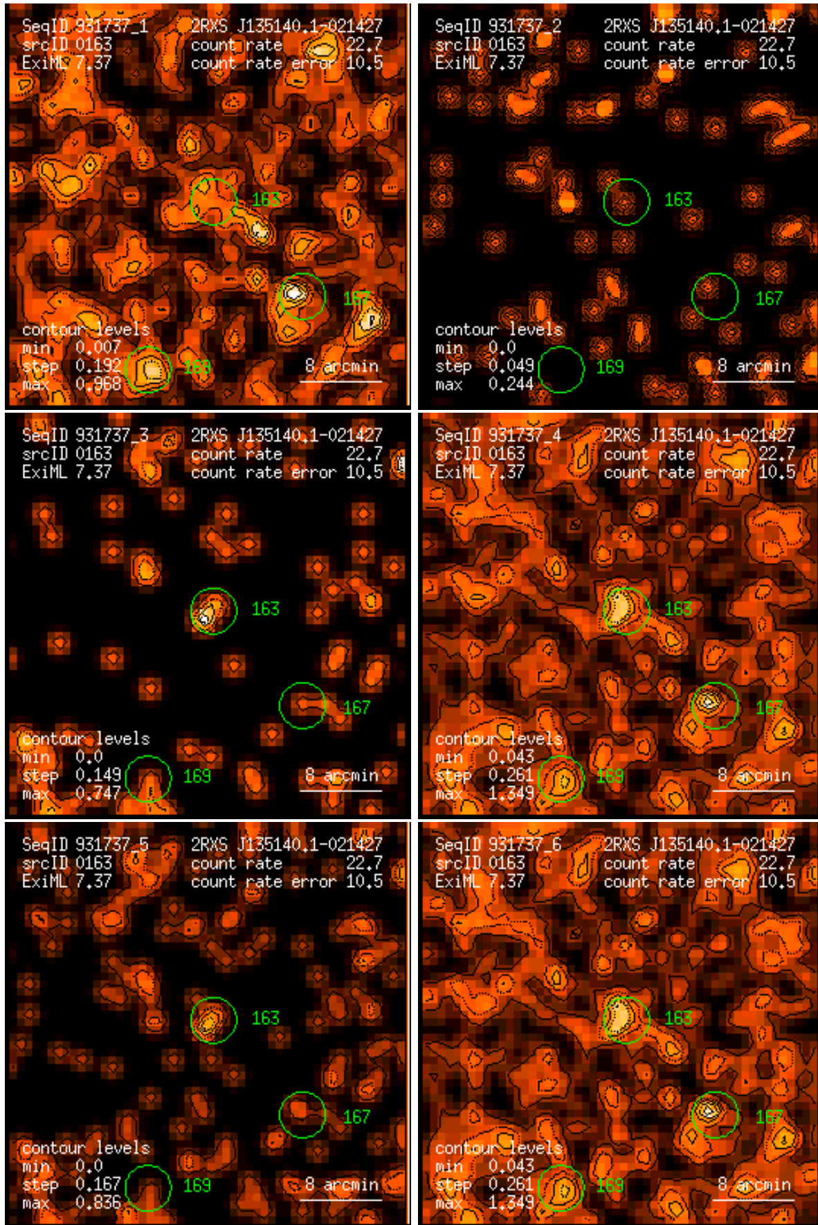
Figure 163: RASS 931737: detection 0163: band rate images, Gaussian filter: (1) PSPC channels 11 – 41, (2) 52 – 90, (3) 91 – 201, (4) 11 – 235, (5) 52 – 201, (6) 11 – 201. Broad band rates in counts/ks. Band rate contour levels in counts/ks/arcmin 2 .
