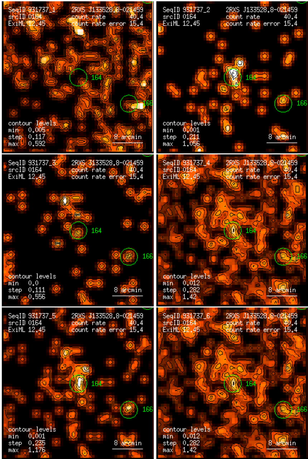
Figure 164: RASS 931737: detection 0164: band rate images, Gaussian filter: (1) PSPC channels 11 – 41, (2) 52 – 90, (3) 91 – 201, (4) 11 – 235, (5) 52 – 201, (6) 11 – 201. Broad band rates in counts/ks. Band rate contour levels in counts/ks/arcmin 2 .
