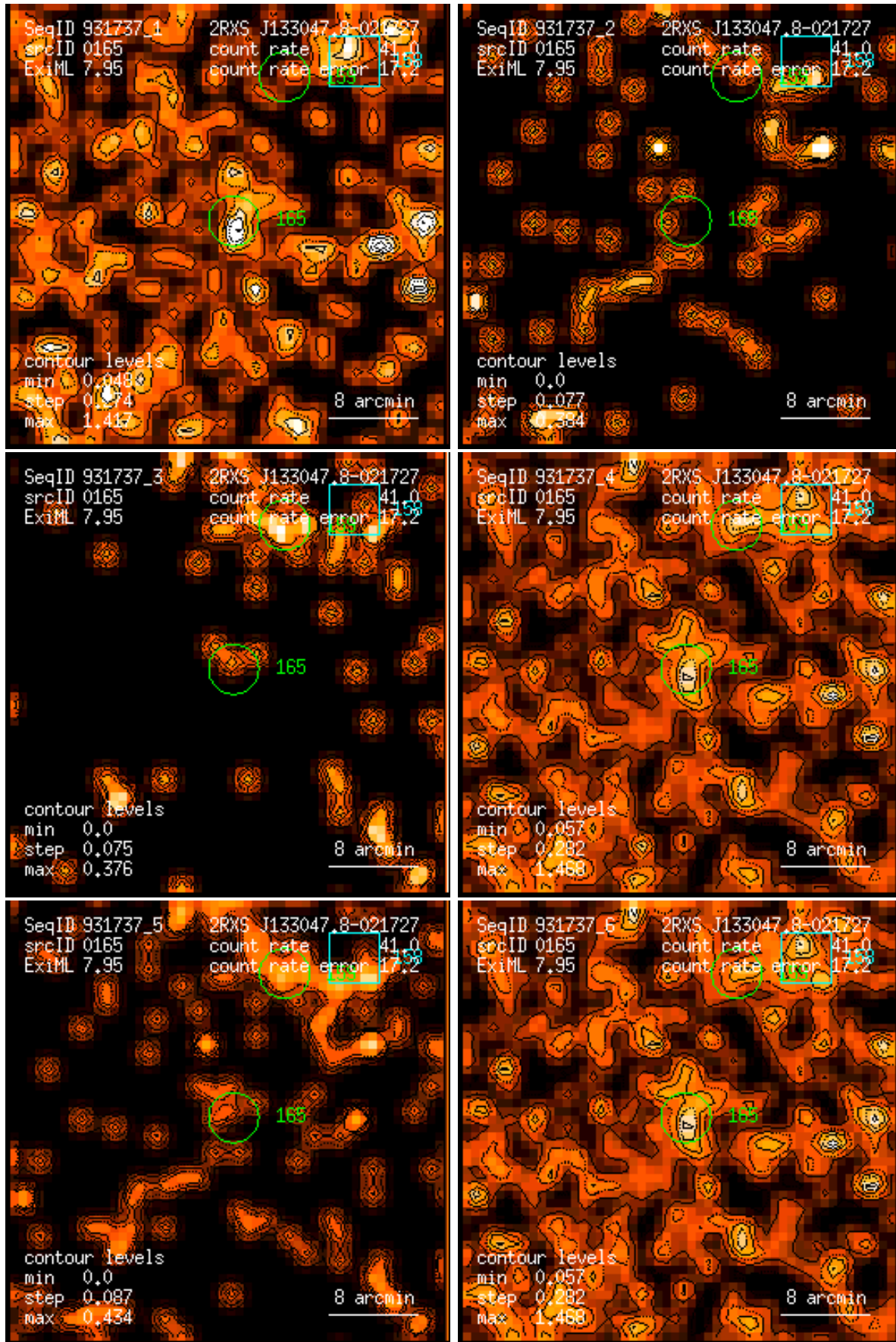
Figure 165: RASS 931737: detection 0165: band rate images, Gaussian filter: (1) PSPC channels 11 – 41, (2) 52 – 90, (3) 91 – 201, (4) 11 – 235, (5) 52 – 201, (6) 11 – 201. Broad band rates in counts/ks. Band rate contour levels in counts/ks/arcmin 2 .
