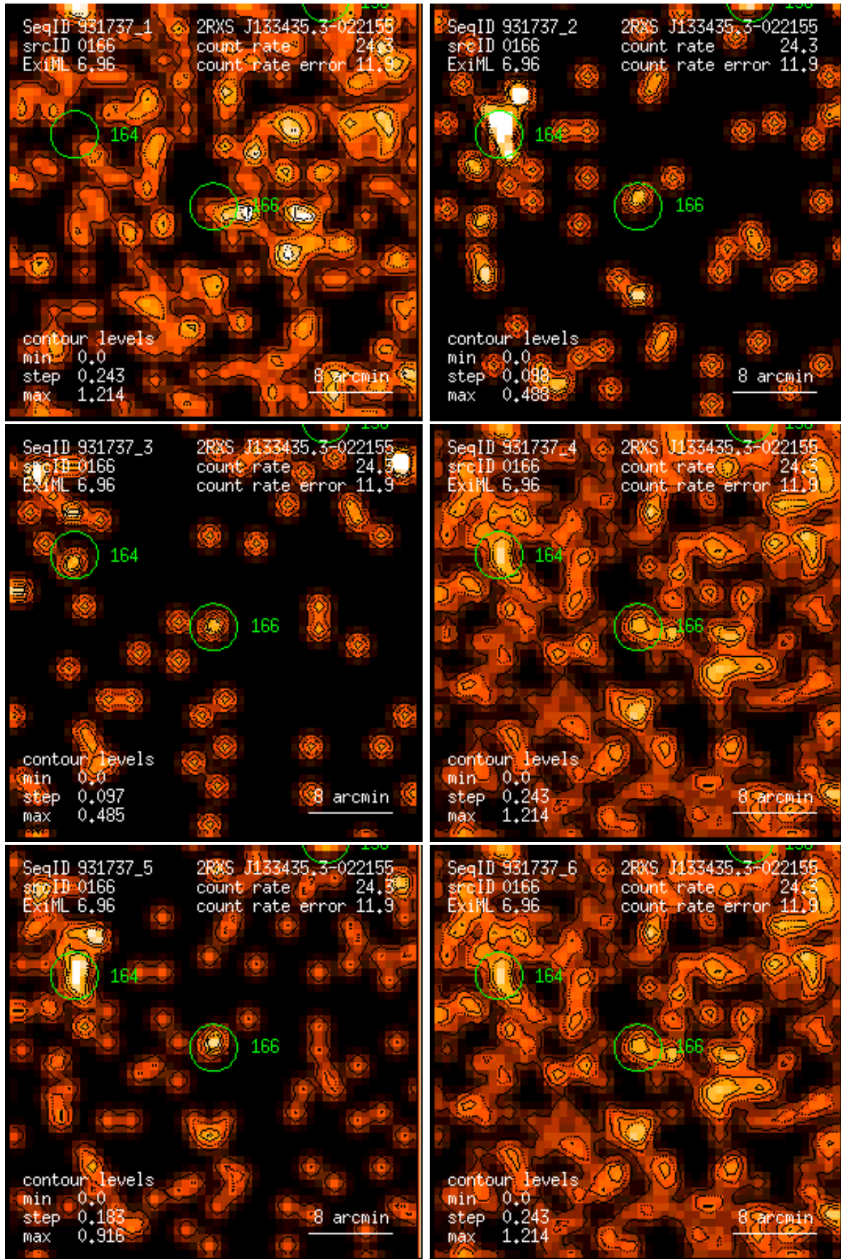
Figure 166: RASS 931737: detection 0166: band rate images, Gaussian filter: (1) PSPC channels 11 – 41, (2) 52 – 90, (3) 91 – 201, (4) 11 – 235, (5) 52 – 201, (6) 11 – 201. Broad band rates in counts/ks. Band rate contour levels in counts/ks/arcmin 2 .
