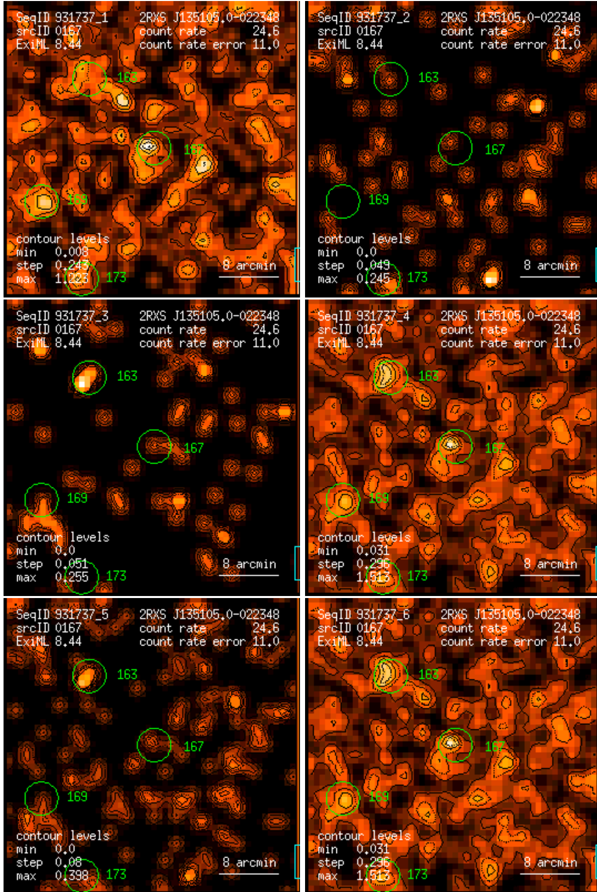
Figure 167: RASS 931737: detection 0167: band rate images, Gaussian filter: (1) PSPC channels 11 – 41, (2) 52 – 90, (3) 91 – 201, (4) 11 – 235, (5) 52 – 201, (6) 11 – 201. Broad band rates in counts/ks. Band rate contour levels in counts/ks/arcmin 2 .
