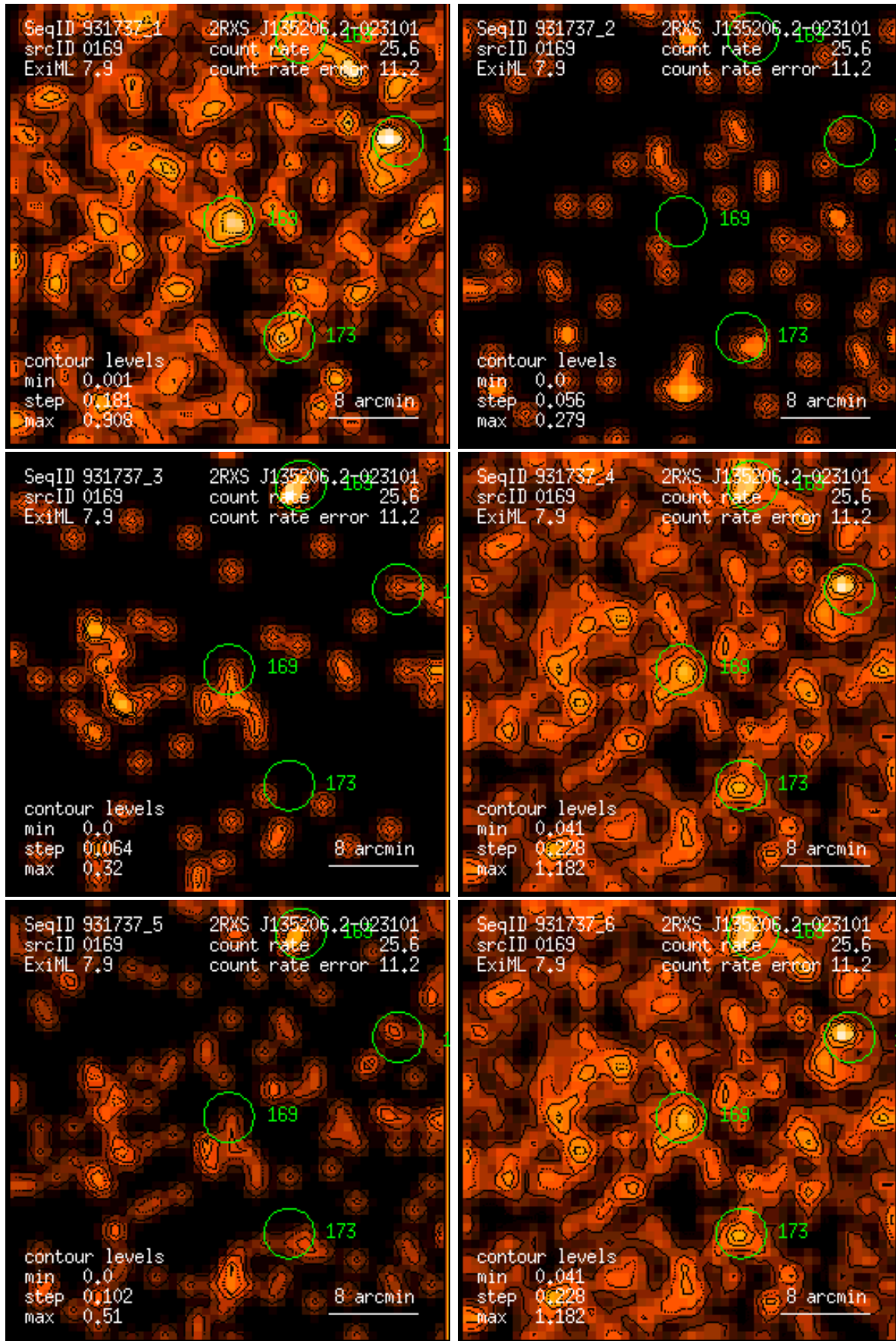
Figure 169: RASS 931737: detection 0169: band rate images, Gaussian filter: (1) PSPC channels 11 – 41, (2) 52 – 90, (3) 91 – 201, (4) 11 – 235, (5) 52 – 201, (6) 11 – 201. Broad band rates in counts/ks. Band rate contour levels in counts/ks/arcmin 2 .
