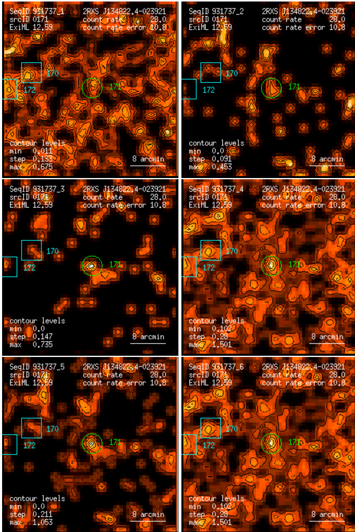
Figure 171: RASS 931737: detection 0171: band rate images, Gaussian filter: (1) PSPC channels 11 – 41, (2) 52 – 90, (3) 91 – 201, (4) 11 – 235, (5) 52 – 201, (6) 11 – 201. Broad band rates in counts/ks. Band rate contour levels in counts/ks/arcmin 2 .
