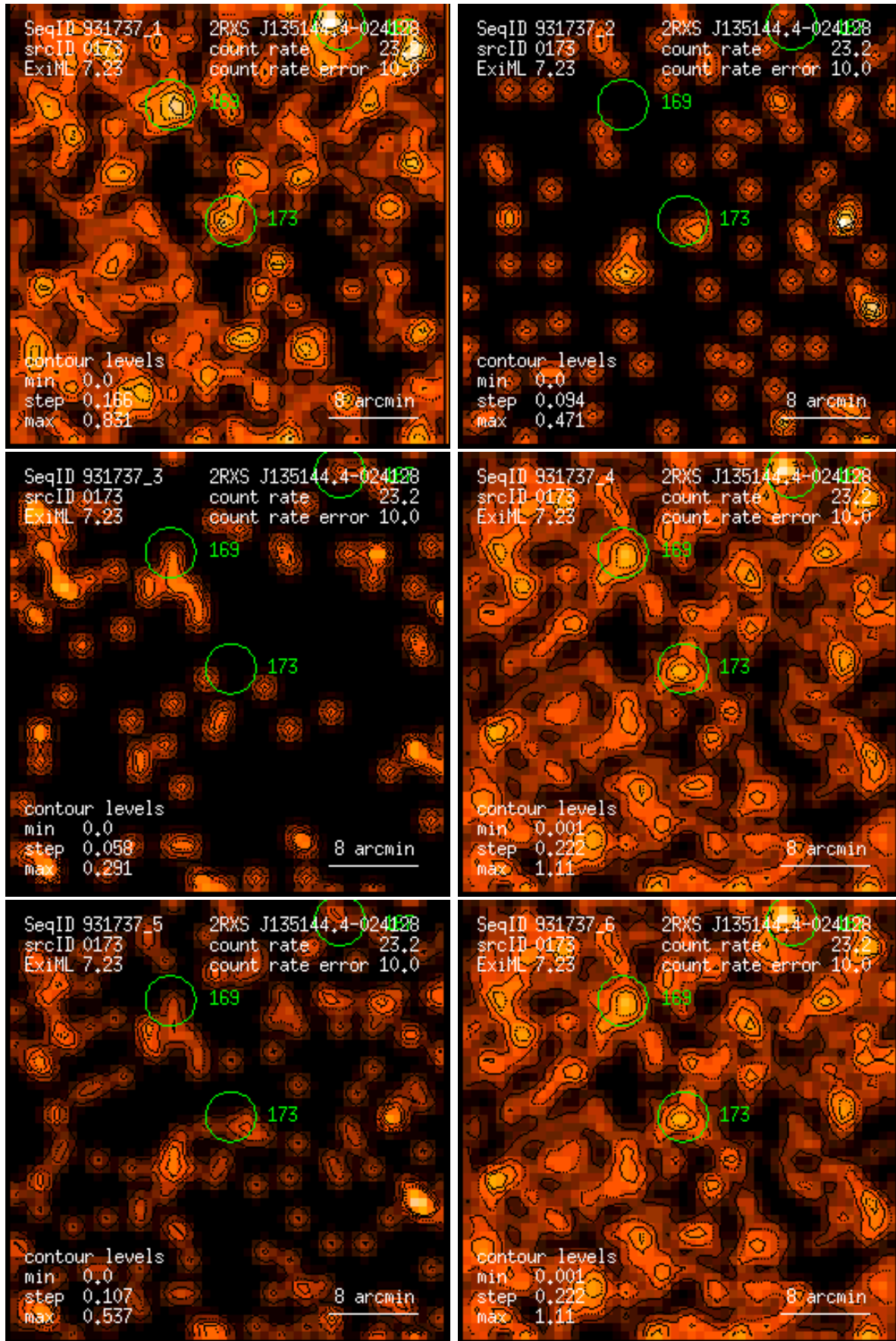
Figure 173: RASS 931737: detection 0173: band rate images, Gaussian filter: (1) PSPC channels 11 – 41, (2) 52 – 90, (3) 91 – 201, (4) 11 – 235, (5) 52 – 201, (6) 11 – 201. Broad band rates in counts/ks. Band rate contour levels in counts/ks/arcmin 2 .
