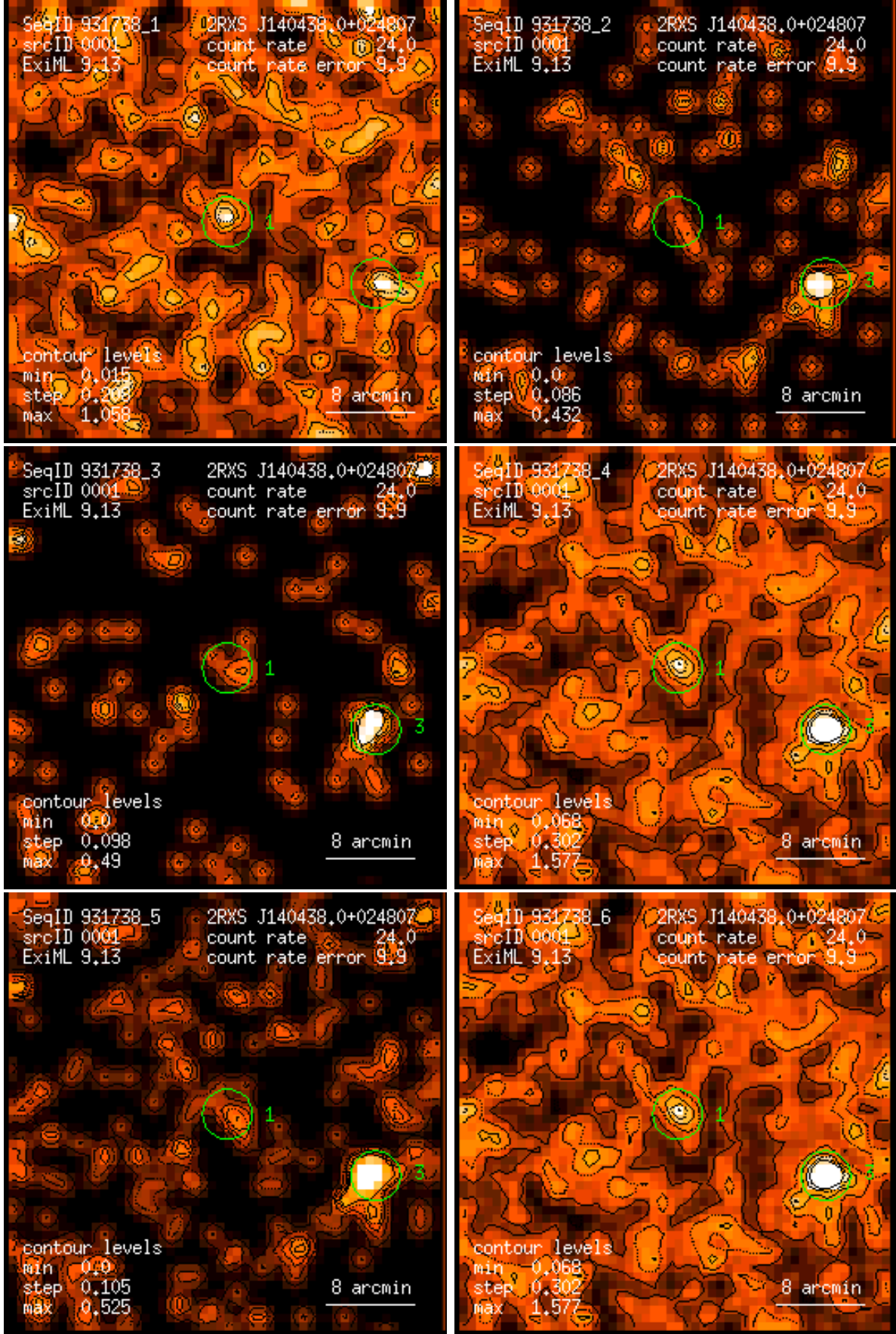
Figure 1: RASS 931738: detection 0001: band rate images, Gaussian filter: (1) PSPC channels 11 – 41, (2) 52 – 90, (3) 91 – 201, (4) 11 – 235, (5) 52 – 201, (6) 11 – 201. Broad band rates in counts/ks. Band rate contour levels in counts/ks/arcmin 2 .
