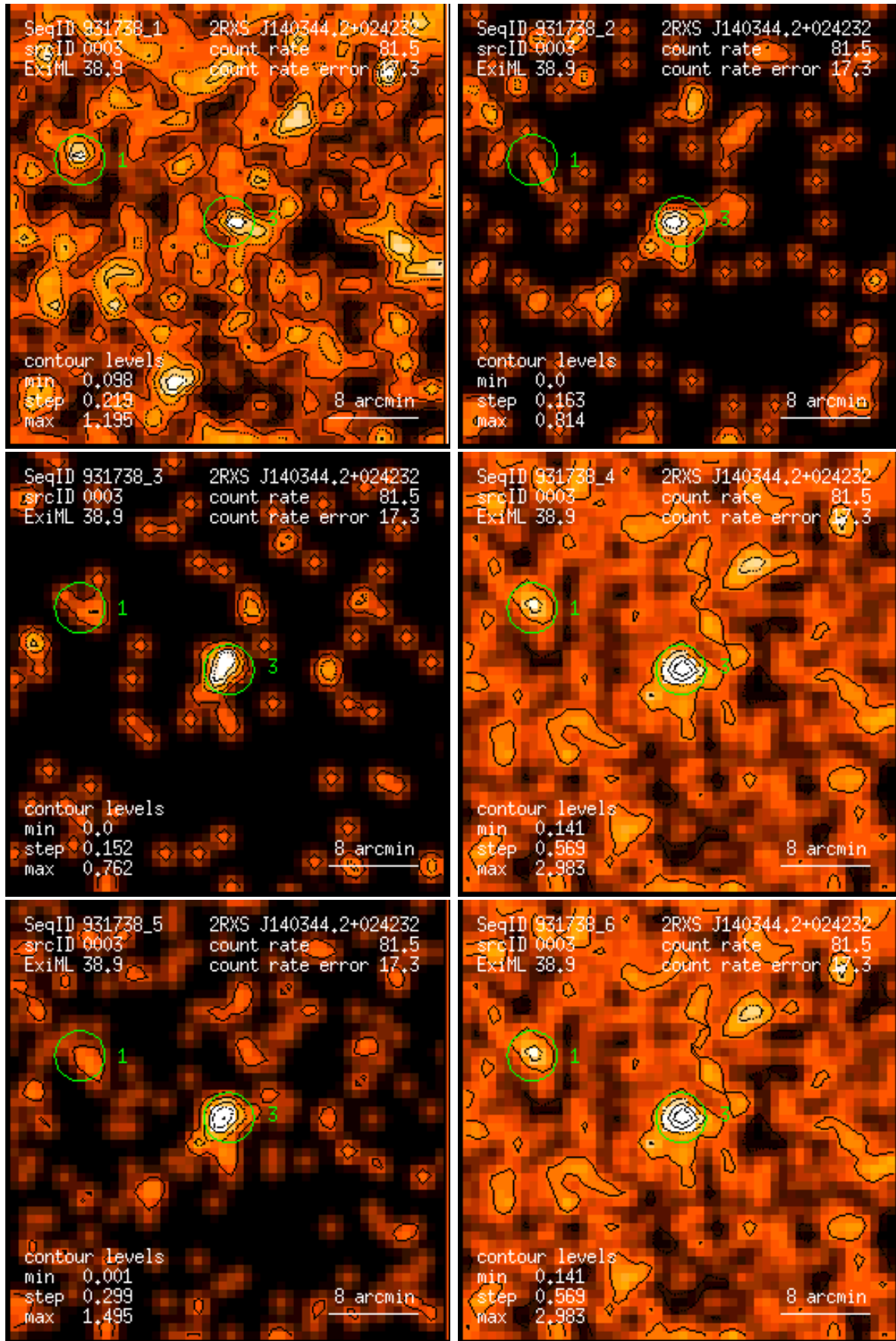
Figure 3: RASS 931738: detection 0003: band rate images, Gaussian filter: (1) PSPC channels 11 – 41, (2) 52 – 90, (3) 91 – 201, (4) 11 – 235, (5) 52 – 201, (6) 11 – 201. Broad band rates in counts/ks. Band rate contour levels in counts/ks/arcmin 2 .
