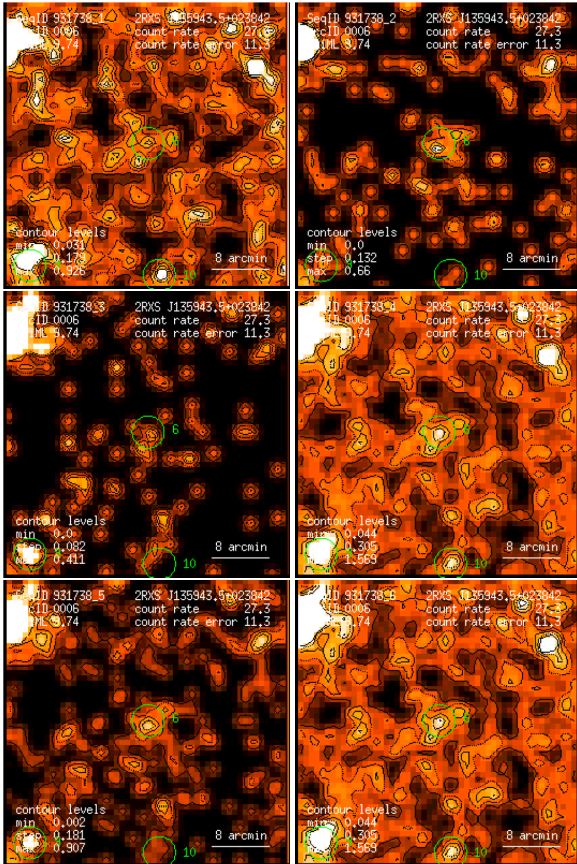
Figure 6: RASS 931738: detection 0006: band rate images, Gaussian filter: (1) PSPC channels 11 – 41, (2) 52 – 90, (3) 91 – 201, (4) 11 – 235, (5) 52 – 201, (6) 11 – 201. Broad band rates in counts/ks. Band rate contour levels in counts/ks/arcmin 2 .
